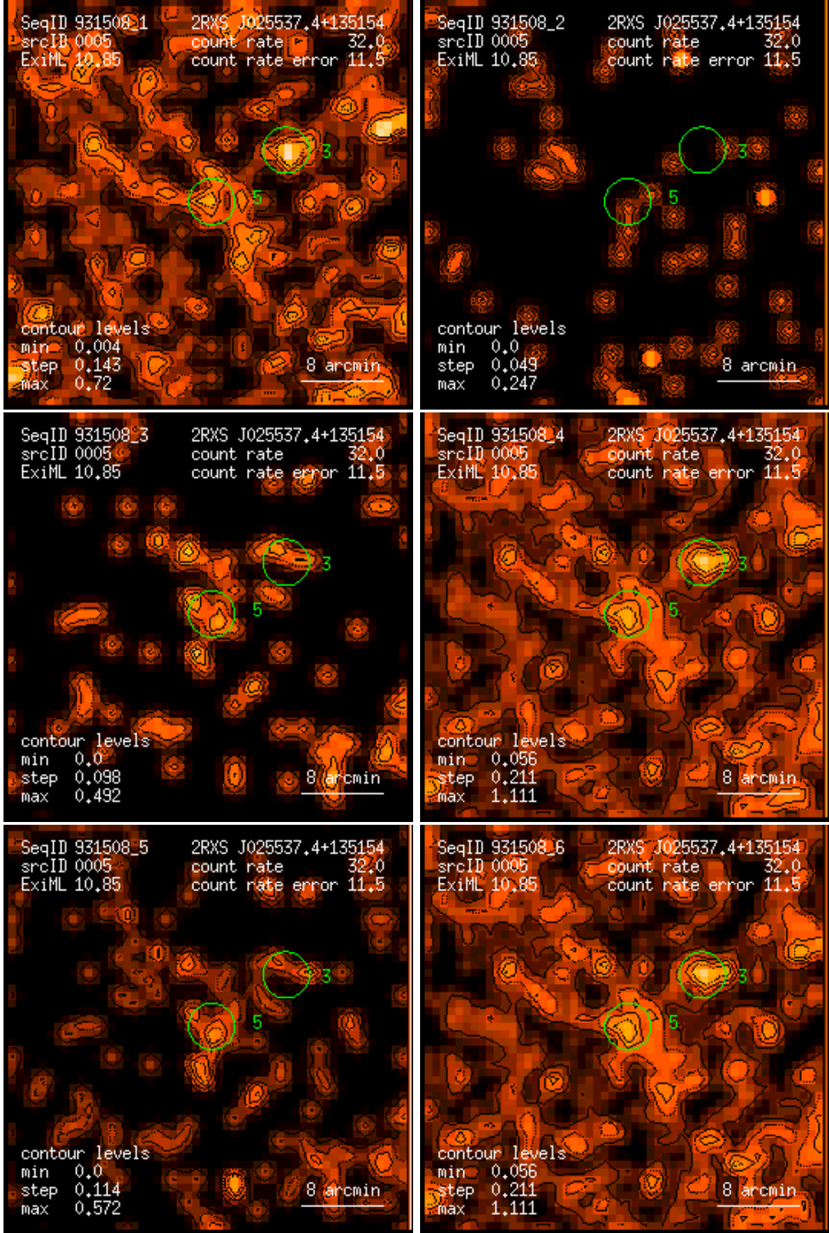
Figure 5: RASS 931508: detection 0005: band rate images, Gaussian filter: (1) PSPC channels 11 – 41, (2) 52 – 90, (3) 91 – 201, (4) 11 – 235, (5) 52 – 201, (6) 11 – 201. Broad band rates in counts/ks. Band rate contour levels in counts/ks/arcmin 2 .
