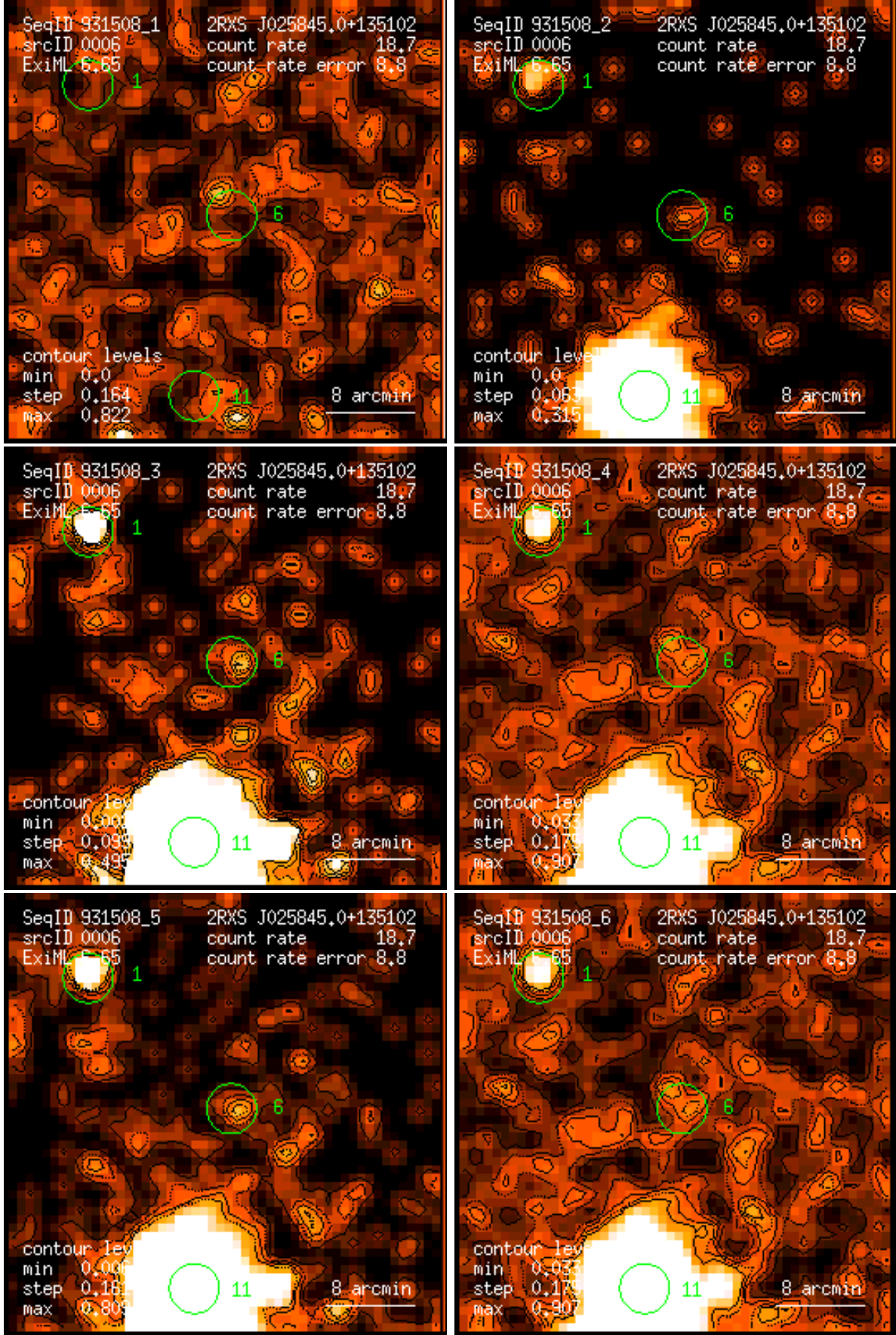
Figure 6: RASS 931508: detection 0006: band rate images, Gaussian filter: (1) PSPC channels 11 – 41, (2) 52 – 90, (3) 91 – 201, (4) 11 – 235, (5) 52 – 201, (6) 11 – 201. Broad band rates in counts/ks. Band rate contour levels in counts/ks/arcmin 2 .
