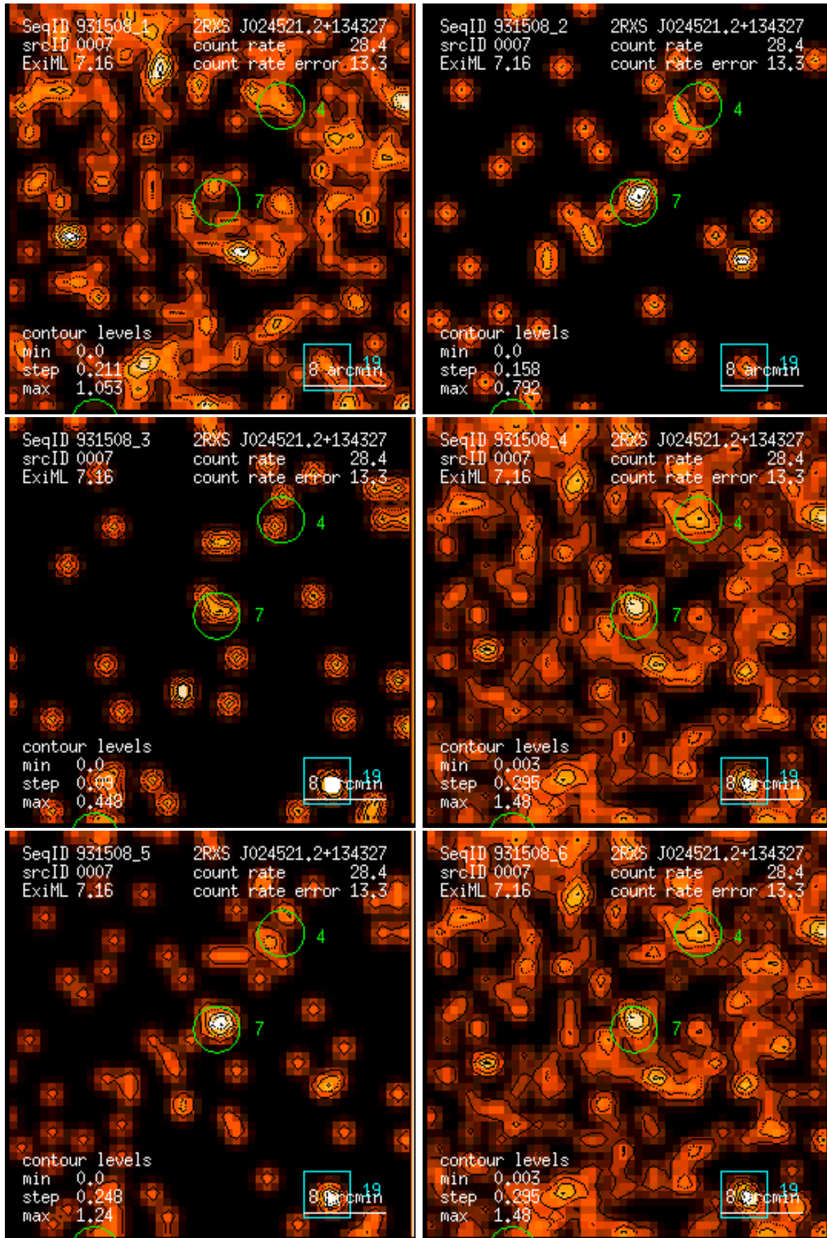
Figure 7: RASS 931508: detection 0007: band rate images, Gaussian filter: (1) PSPC channels 11 – 41, (2) 52 – 90, (3) 91 – 201, (4) 11 – 235, (5) 52 – 201, (6) 11 – 201. Broad band rates in counts/ks. Band rate contour levels in counts/ks/arcmin 2 .
