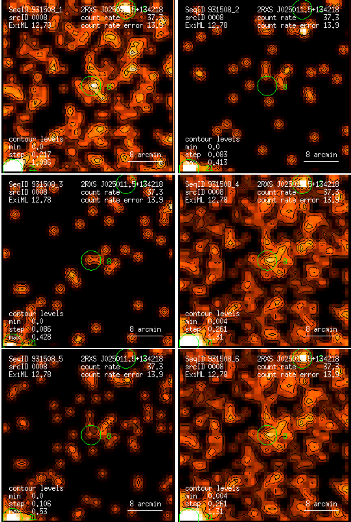
Figure 8: RASS 931508: detection 0008: band rate images, Gaussian filter: (1) PSPC channels 11 – 41, (2) 52 – 90, (3) 91 – 201, (4) 11 – 235, (5) 52 – 201, (6) 11 – 201. Broad band rates in counts/ks. Band rate contour levels in counts/ks/arcmin 2 .
