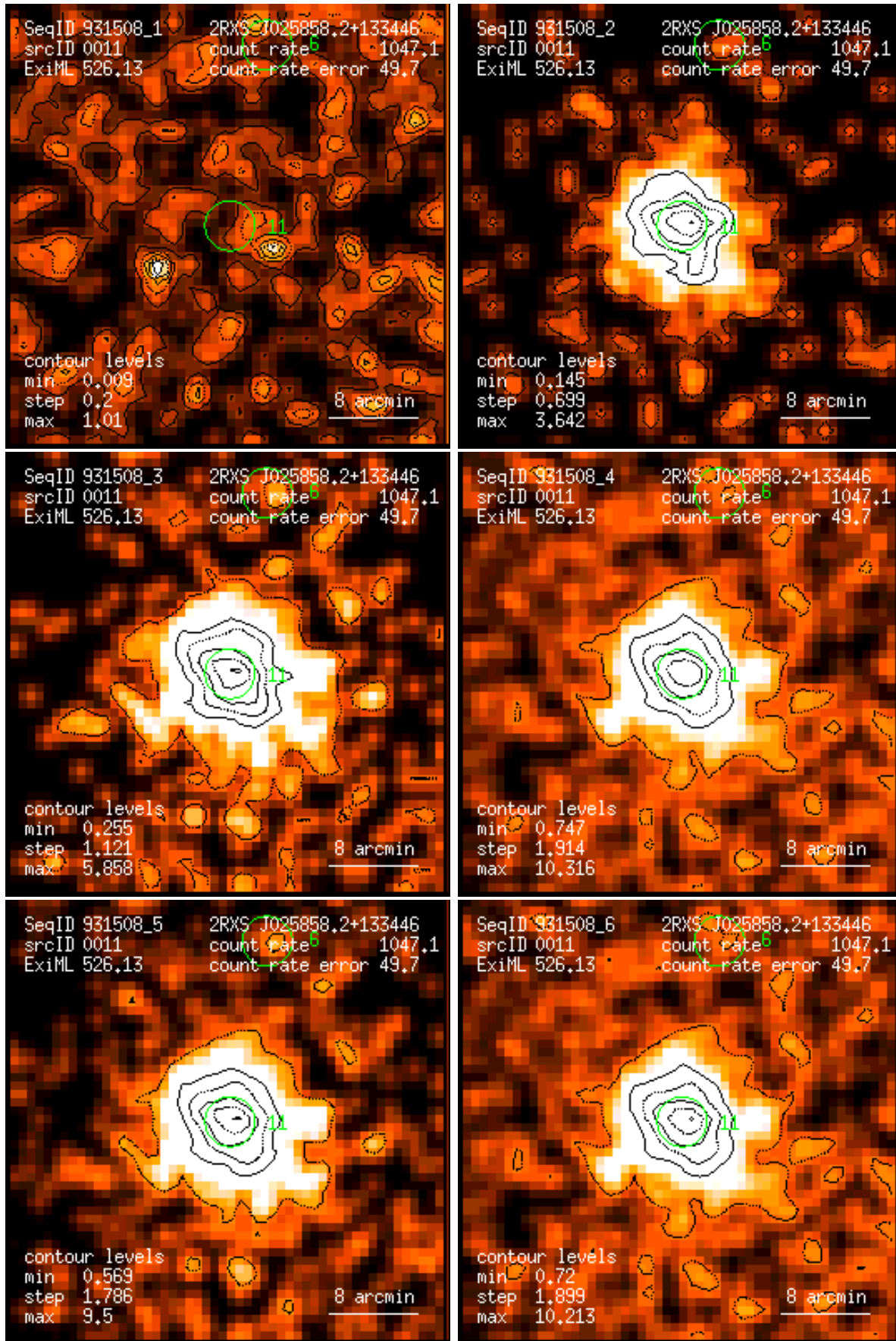
Figure 11: RASS 931508: detection 0011: band rate images, Gaussian filter: (1) PSPC channels 11 – 41, (2) 52 – 90, (3) 91 – 201, (4) 11 – 235, (5) 52 – 201, (6) 11 – 201. Broad band rates in counts/ks. Band rate contour levels in counts/ks/arcmin 2 .
