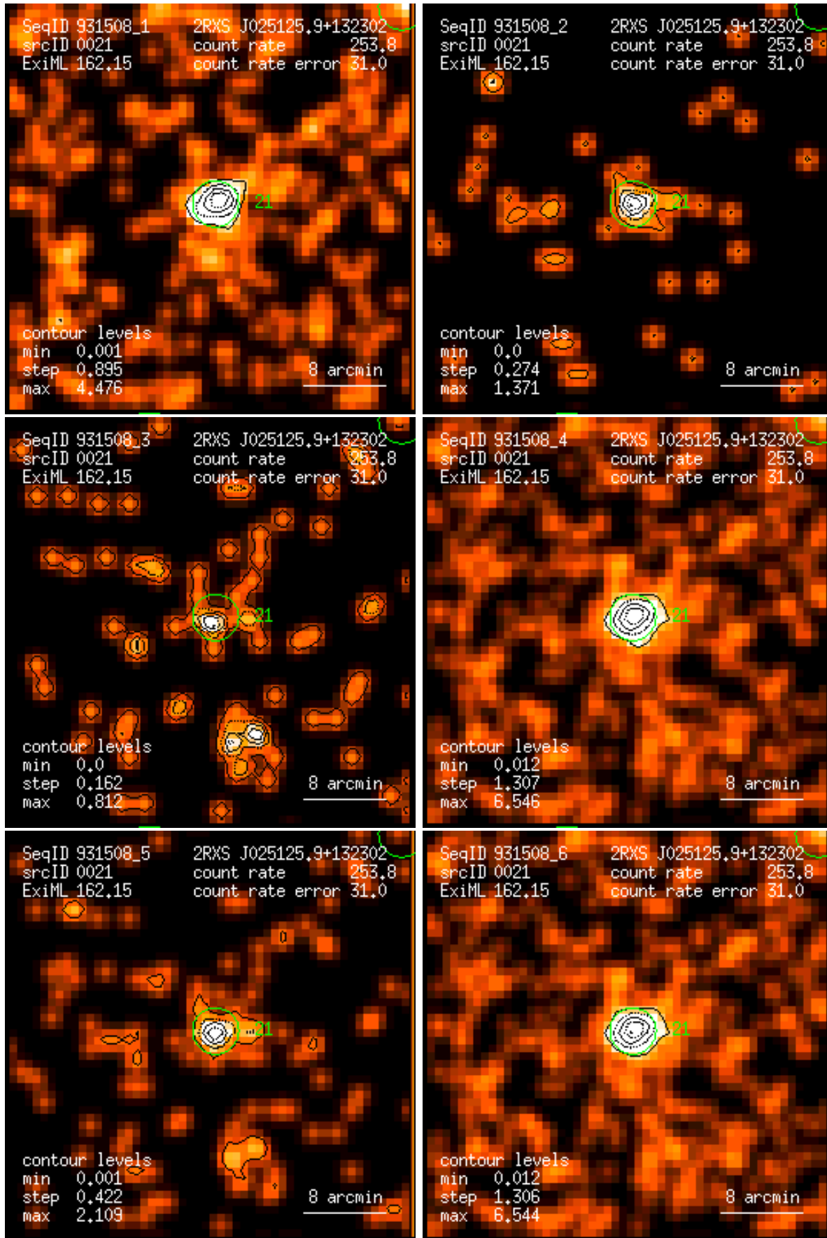
Figure 21: RASS 931508: detection 0021: band rate images, Gaussian filter: (1) PSPC channels 11 – 41, (2) 52 – 90, (3) 91 – 201, (4) 11 – 235, (5) 52 – 201, (6) 11 – 201. Broad band rates in counts/ks. Band rate contour levels in counts/ks/arcmin 2 .
