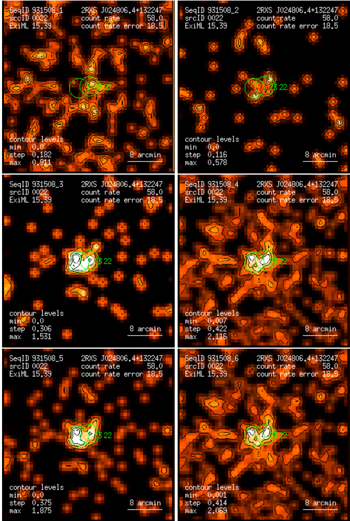
Figure 22: RASS 931508: detection 0022: band rate images, Gaussian filter: (1) PSPC channels 11 – 41, (2) 52 – 90, (3) 91 – 201, (4) 11 – 235, (5) 52 – 201, (6) 11 – 201. Broad band rates in counts/ks. Band rate contour levels in counts/ks/arcmin 2 .
