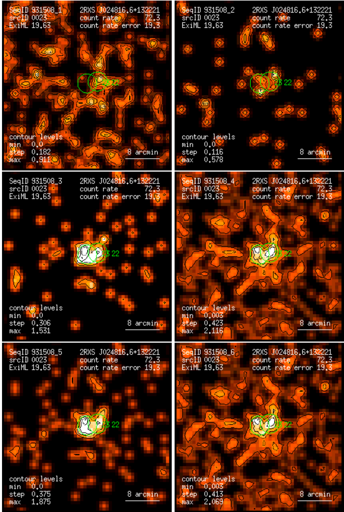
Figure 23: RASS 931508: detection 0023: band rate images, Gaussian filter: (1) PSPC channels 11 – 41, (2) 52 – 90, (3) 91 – 201, (4) 11 – 235, (5) 52 – 201, (6) 11 – 201. Broad band rates in counts/ks. Band rate contour levels in counts/ks/arcmin 2 .
