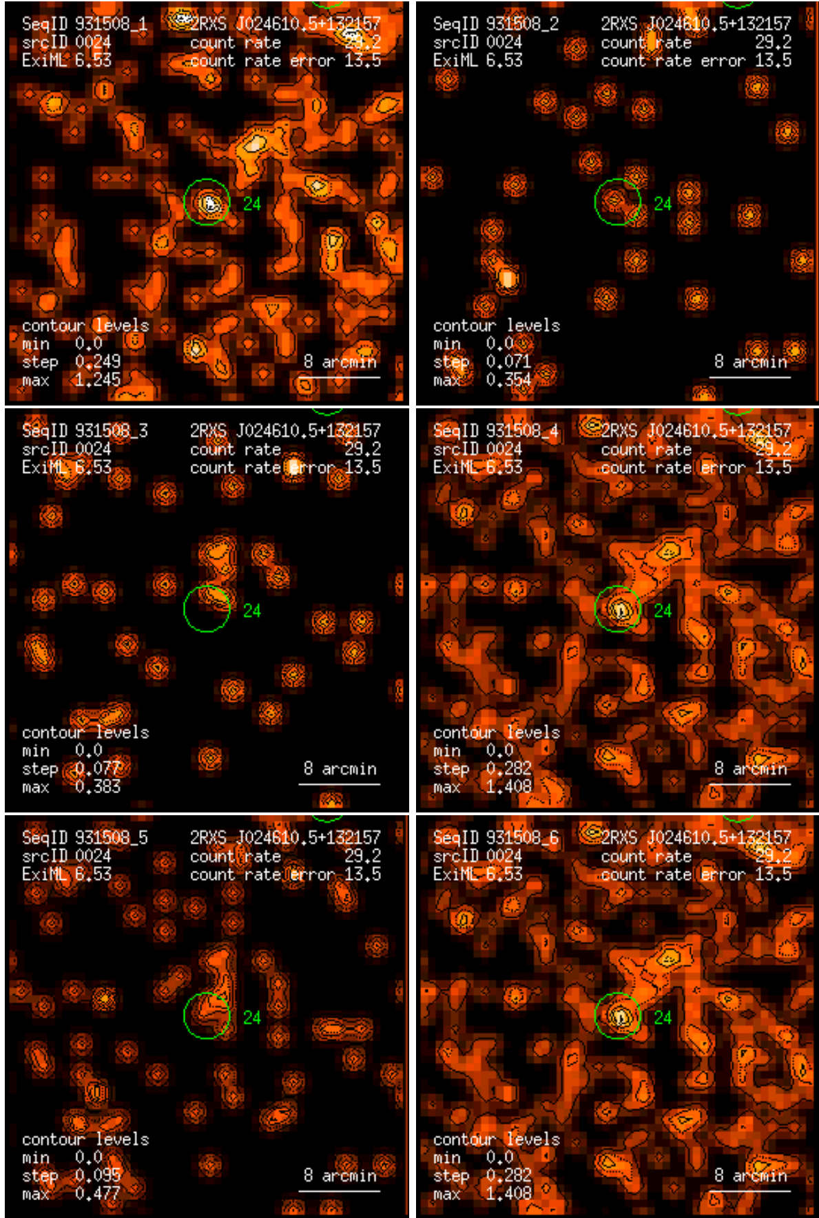
Figure 24: RASS 931508: detection 0024: band rate images, Gaussian filter: (1) PSPC channels 11 – 41, (2) 52 – 90, (3) 91 – 201, (4) 11 – 235, (5) 52 – 201, (6) 11 – 201. Broad band rates in counts/ks. Band rate contour levels in counts/ks/arcmin 2 .
