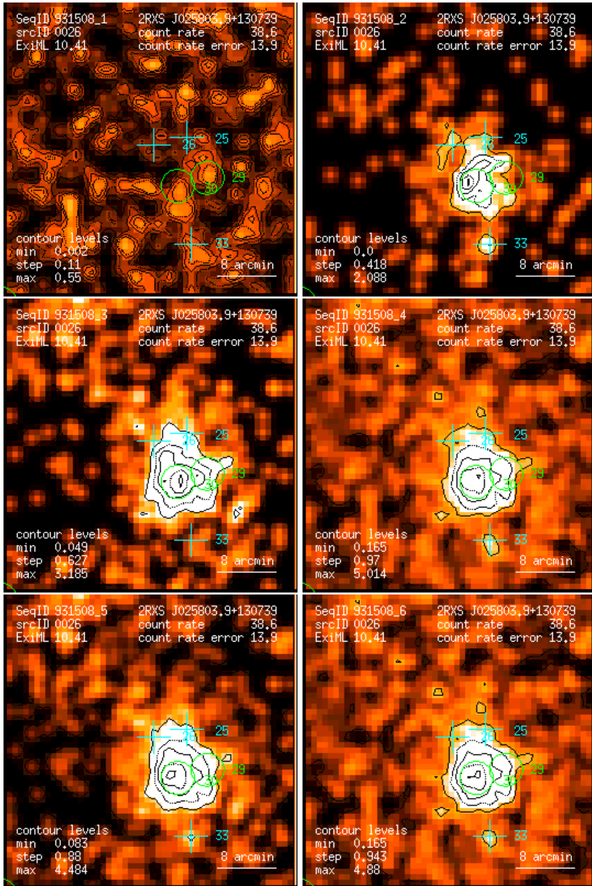
Figure 26: RASS 931508: detection 0026: band rate images, Gaussian filter: (1) PSPC channels 11 – 41, (2) 52 – 90, (3) 91 – 201, (4) 11 – 235, (5) 52 – 201, (6) 11 – 201. Broad band rates in counts/ks. Band rate contour levels in counts/ks/arcmin 2 .
