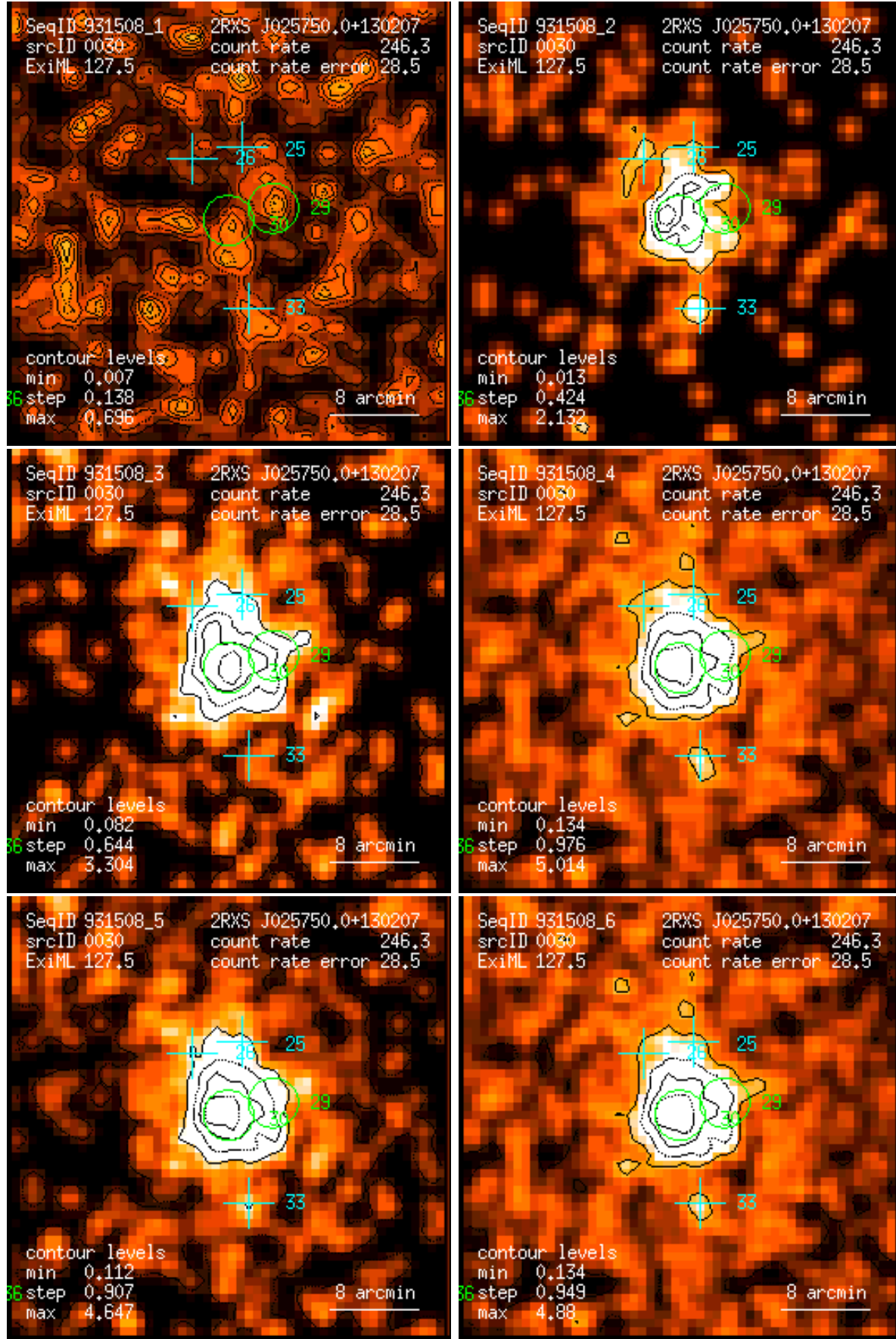
Figure 30: RASS 931508: detection 0030: band rate images, Gaussian filter: (1) PSPC channels 11 – 41, (2) 52 – 90, (3) 91 – 201, (4) 11 – 235, (5) 52 – 201, (6) 11 – 201. Broad band rates in counts/ks. Band rate contour levels in counts/ks/arcmin 2 .
