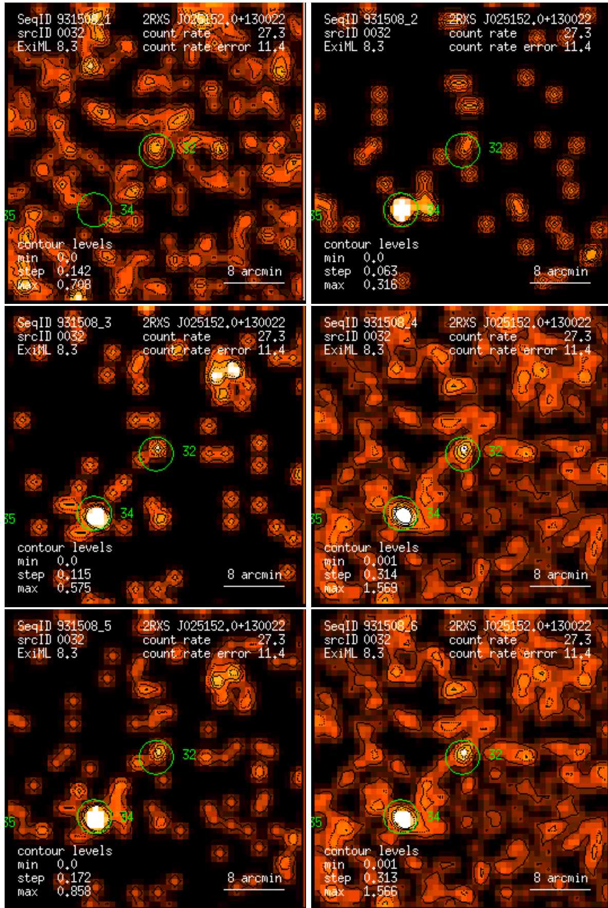
Figure 32: RASS 931508: detection 0032: band rate images, Gaussian filter: (1) PSPC channels 11 – 41, (2) 52 – 90, (3) 91 – 201, (4) 11 – 235, (5) 52 – 201, (6) 11 – 201. Broad band rates in counts/ks. Band rate contour levels in counts/ks/arcmin 2 .
