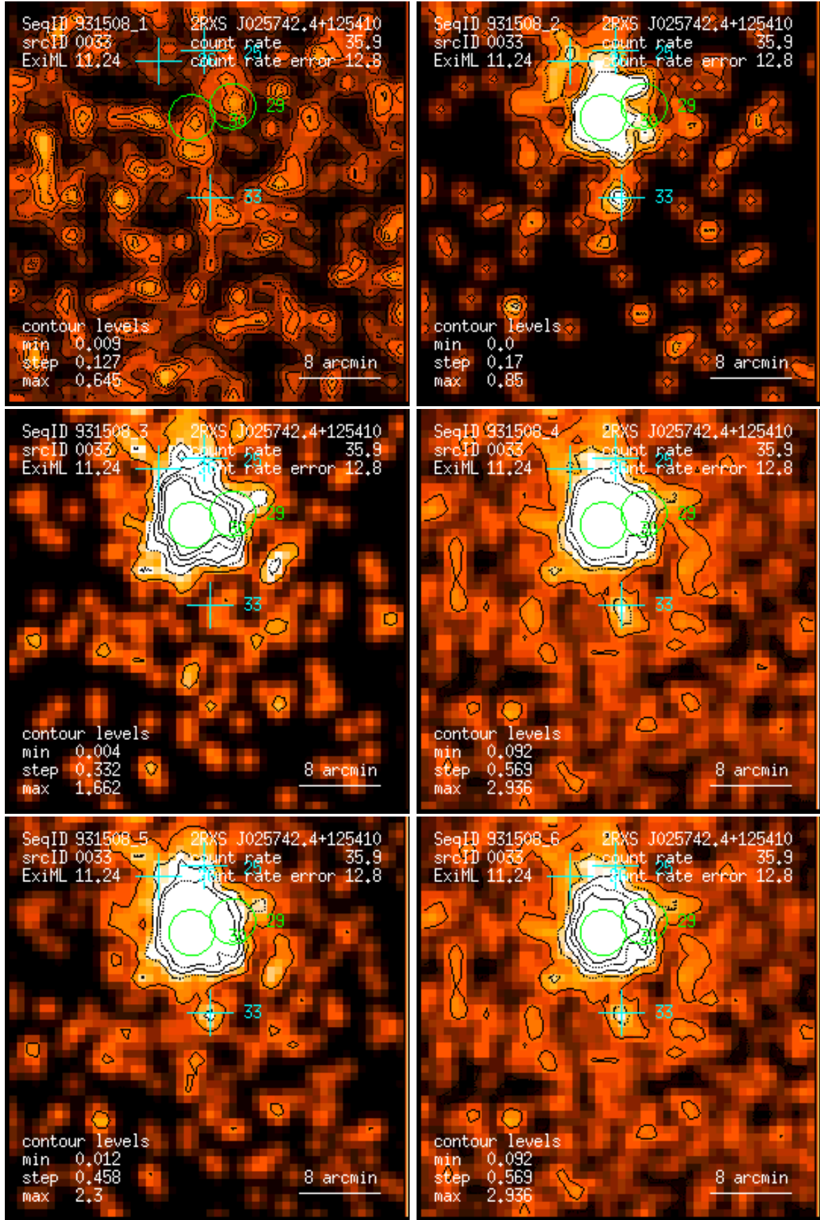
Figure 33: RASS 931508: detection 0033: band rate images, Gaussian filter: (1) PSPC channels 11 – 41, (2) 52 – 90, (3) 91 – 201, (4) 11 – 235, (5) 52 – 201, (6) 11 – 201. Broad band rates in counts/ks. Band rate contour levels in counts/ks/arcmin 2 .
