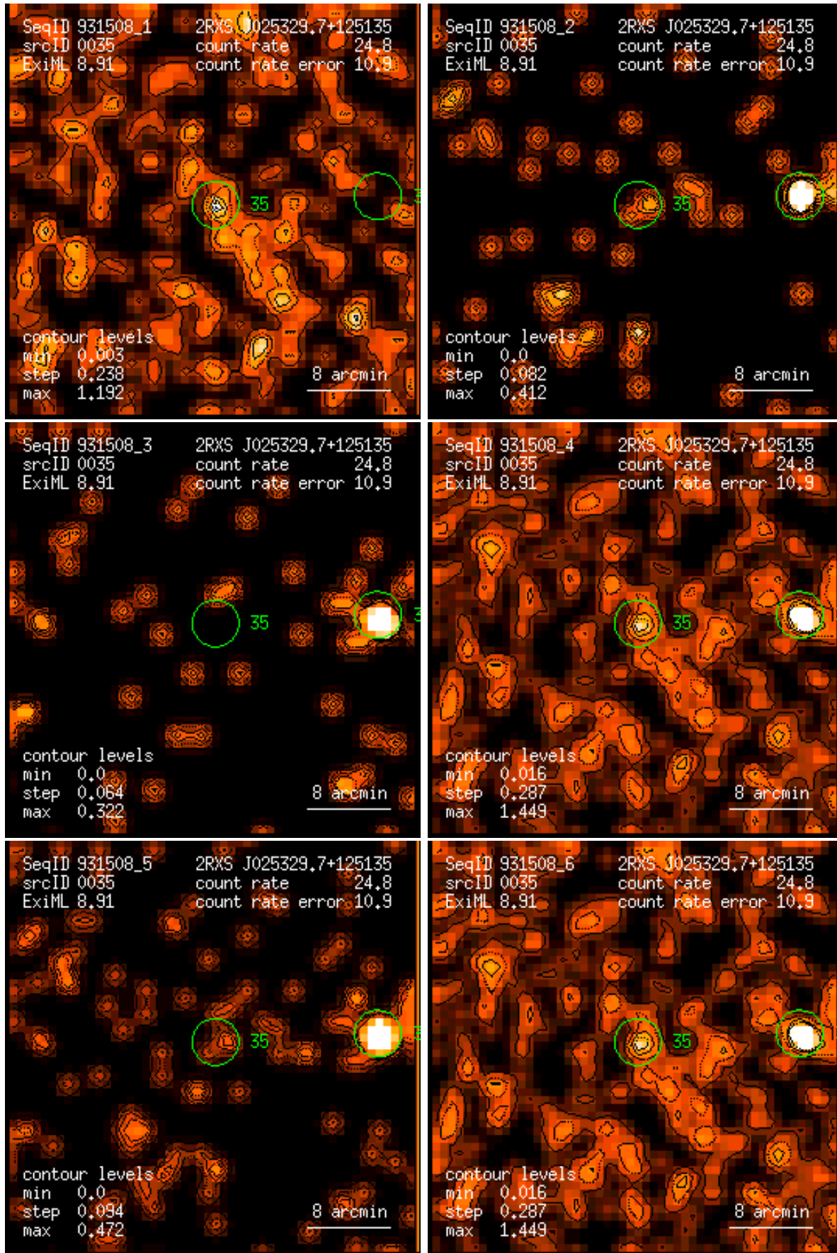
Figure 35: RASS 931508: detection 0035: band rate images, Gaussian filter: (1) PSPC channels 11 – 41, (2) 52 – 90, (3) 91 – 201, (4) 11 – 235, (5) 52 – 201, (6) 11 – 201. Broad band rates in counts/ks. Band rate contour levels in counts/ks/arcmin 2 .
