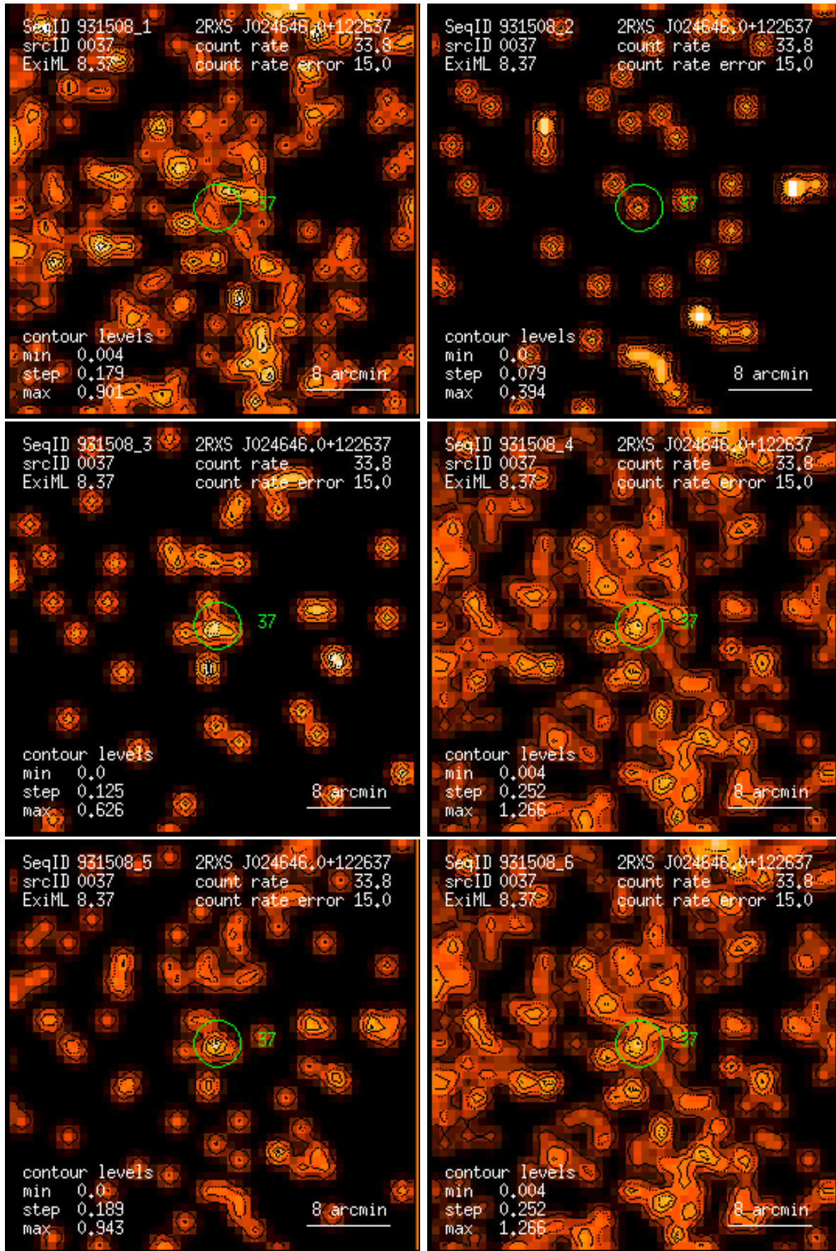
Figure 37: RASS 931508: detection 0037: band rate images, Gaussian filter: (1) PSPC channels 11 – 41, (2) 52 – 90, (3) 91 – 201, (4) 11 – 235, (5) 52 – 201, (6) 11 – 201. Broad band rates in counts/ks. Band rate contour levels in counts/ks/arcmin 2 .
