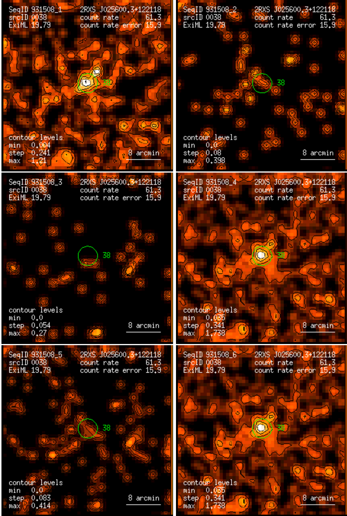
Figure 38: RASS 931508: detection 0038: band rate images, Gaussian filter: (1) PSPC channels 11 – 41, (2) 52 – 90, (3) 91 – 201, (4) 11 – 235, (5) 52 – 201, (6) 11 – 201. Broad band rates in counts/ks. Band rate contour levels in counts/ks/arcmin 2 .
