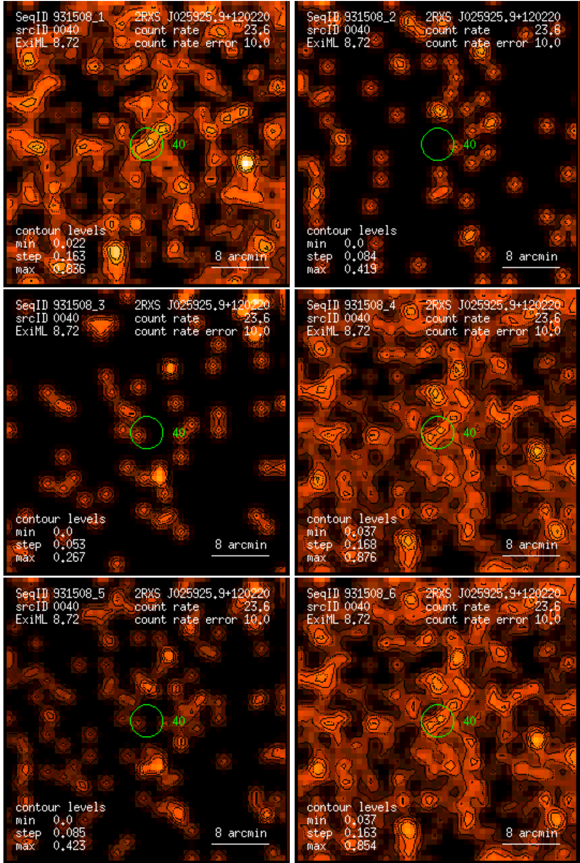
Figure 40: RASS 931508: detection 0040: band rate images, Gaussian filter: (1) PSPC channels 11 – 41, (2) 52 – 90, (3) 91 – 201, (4) 11 – 235, (5) 52 – 201, (6) 11 – 201. Broad band rates in counts/ks. Band rate contour levels in counts/ks/arcmin 2 .
