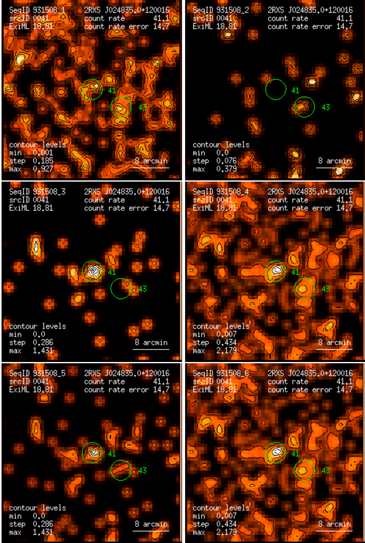
Figure 41: RASS 931508: detection 0041: band rate images, Gaussian filter: (1) PSPC channels 11 – 41, (2) 52 – 90, (3) 91 – 201, (4) 11 – 235, (5) 52 – 201, (6) 11 – 201. Broad band rates in counts/ks. Band rate contour levels in counts/ks/arcmin 2 .
