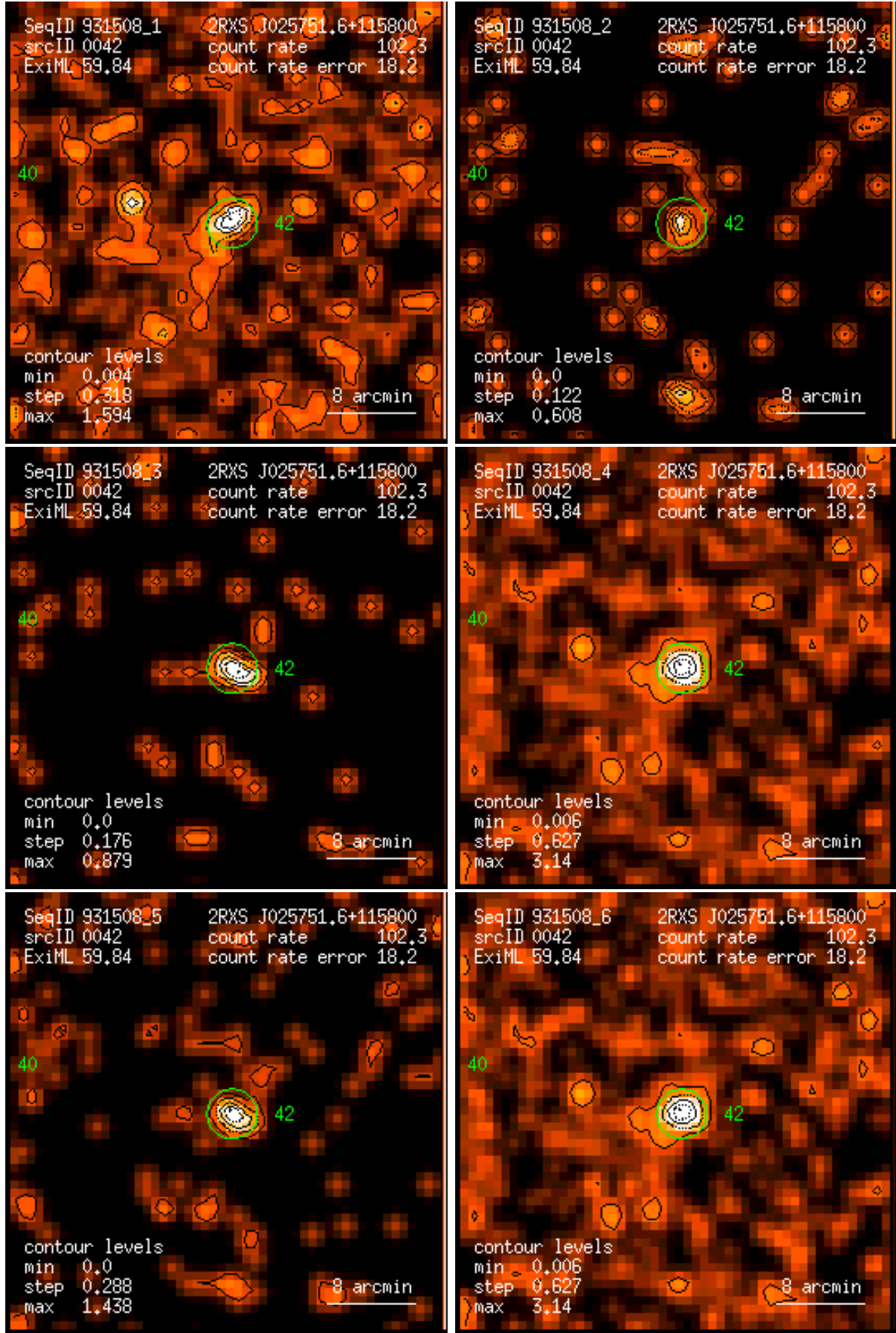
Figure 42: RASS 931508: detection 0042: band rate images, Gaussian filter: (1) PSPC channels 11 – 41, (2) 52 – 90, (3) 91 – 201, (4) 11 – 235, (5) 52 – 201, (6) 11 – 201. Broad band rates in counts/ks. Band rate contour levels in counts/ks/arcmin 2 .
