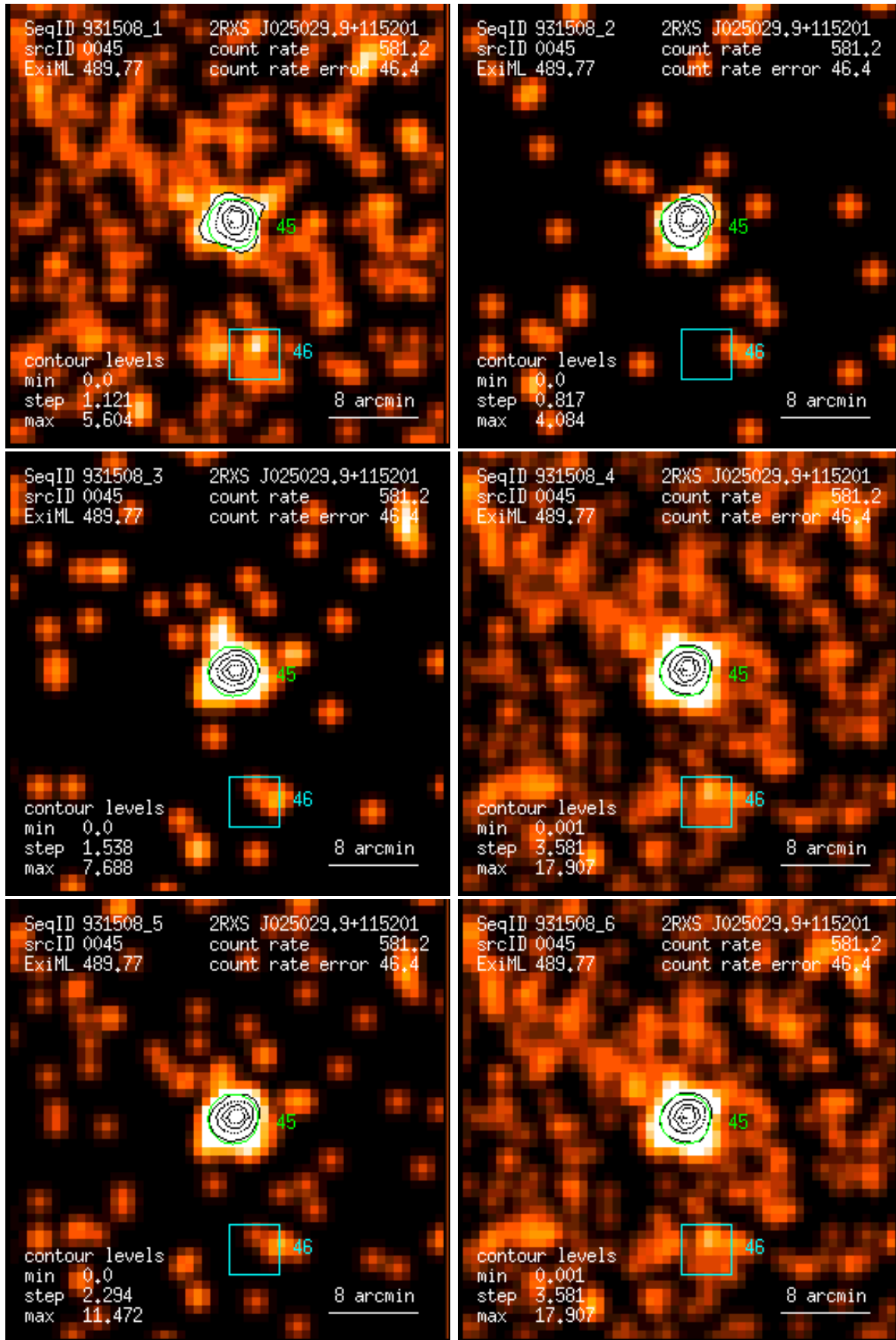
Figure 45: RASS 931508: detection 0045: band rate images, Gaussian filter: (1) PSPC channels 11 – 41, (2) 52 – 90, (3) 91 – 201, (4) 11 – 235, (5) 52 – 201, (6) 11 – 201. Broad band rates in counts/ks. Band rate contour levels in counts/ks/arcmin 2 .
