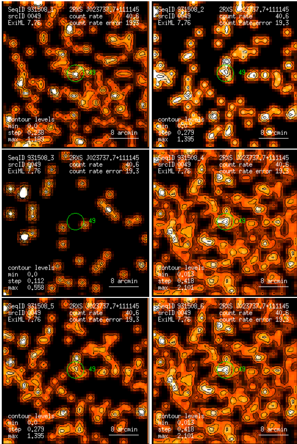
Figure 49: RASS 931508: detection 0049: band rate images, Gaussian filter: (1) PSPC channels 11 – 41, (2) 52 – 90, (3) 91 – 201, (4) 11 – 235, (5) 52 – 201, (6) 11 – 201. Broad band rates in counts/ks. Band rate contour levels in counts/ks/arcmin 2 .
