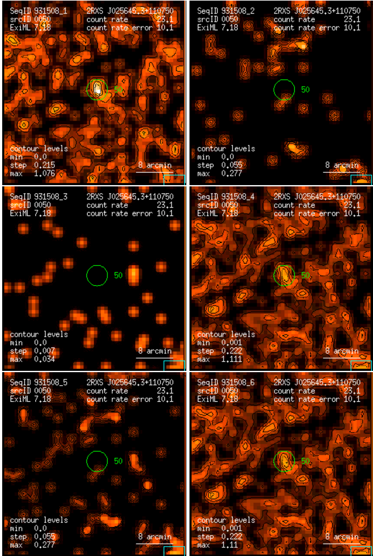
Figure 50: RASS 931508: detection 0050: band rate images, Gaussian filter: (1) PSPC channels 11 – 41, (2) 52 – 90, (3) 91 – 201, (4) 11 – 235, (5) 52 – 201, (6) 11 – 201. Broad band rates in counts/ks. Band rate contour levels in counts/ks/arcmin 2 .
