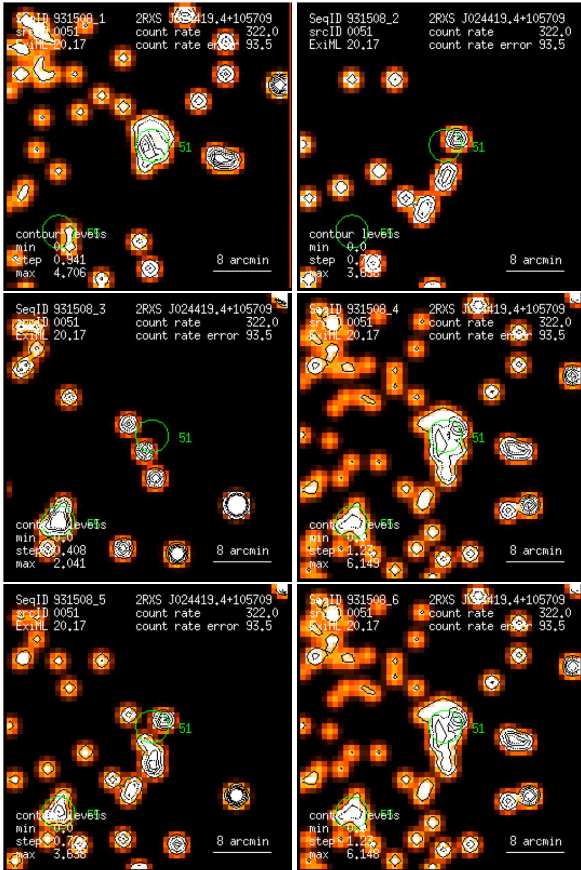
Figure 51: RASS 931508: detection 0051: band rate images, Gaussian filter: (1) PSPC channels 11 – 41, (2) 52 – 90, (3) 91 – 201, (4) 11 – 235, (5) 52 – 201, (6) 11 – 201. Broad band rates in counts/ks. Band rate contour levels in counts/ks/arcmin 2 .
