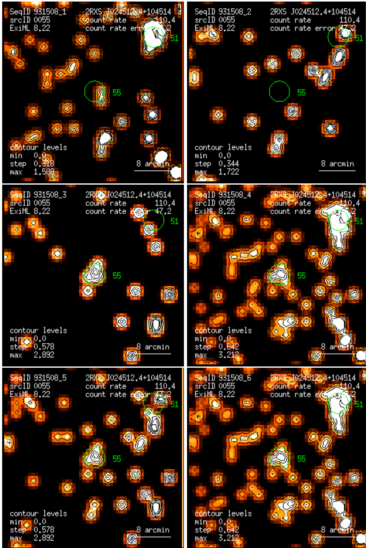
Figure 55: RASS 931508: detection 0055: band rate images, Gaussian filter: (1) PSPC channels 11 – 41, (2) 52 – 90, (3) 91 – 201, (4) 11 – 235, (5) 52 – 201, (6) 11 – 201. Broad band rates in counts/ks. Band rate contour levels in counts/ks/arcmin 2 .
