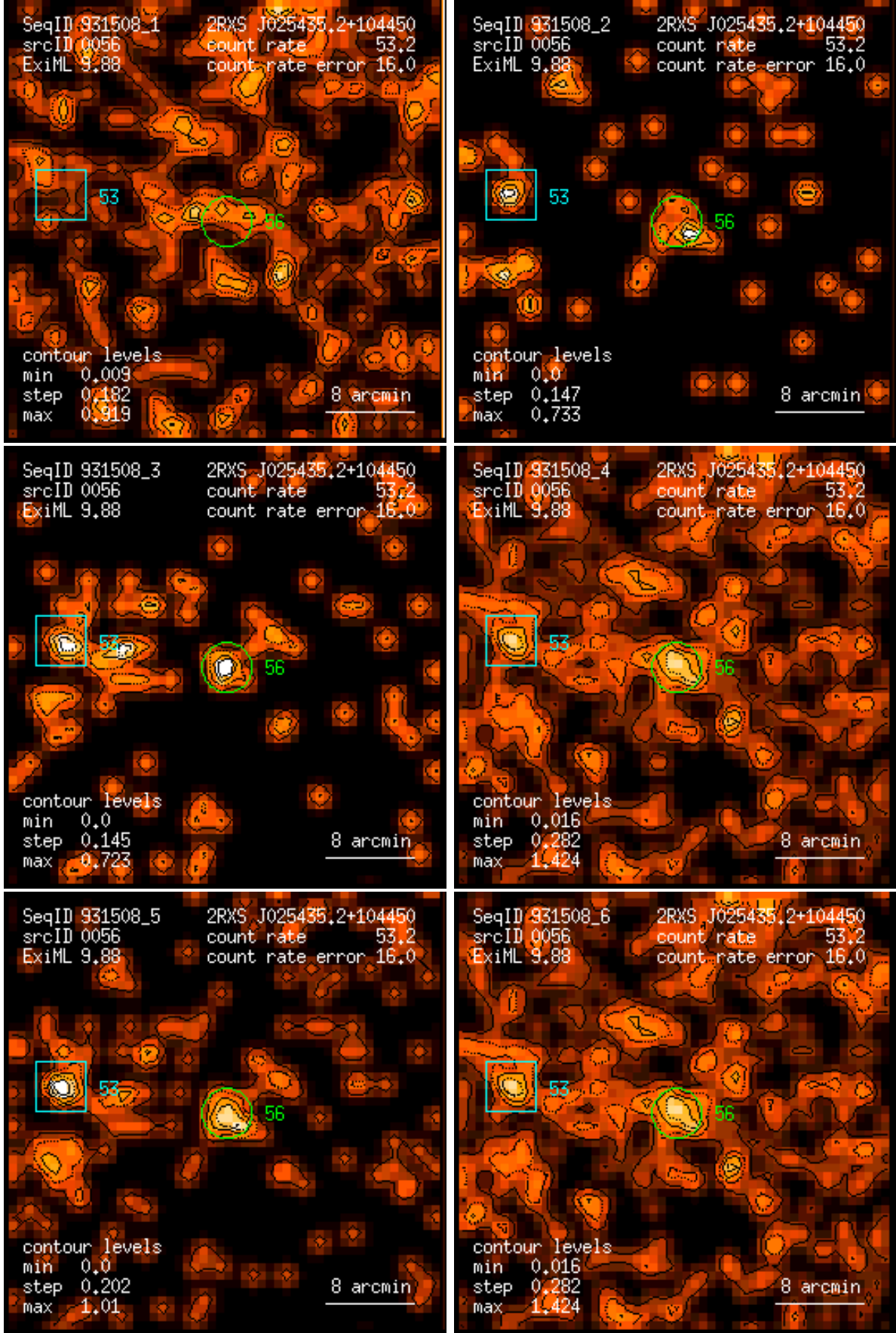
Figure 56: RASS 931508: detection 0056: band rate images, Gaussian filter: (1) PSPC channels 11 – 41, (2) 52 – 90, (3) 91 – 201, (4) 11 – 235, (5) 52 – 201, (6) 11 – 201. Broad band rates in counts/ks. Band rate contour levels in counts/ks/arcmin 2 .
