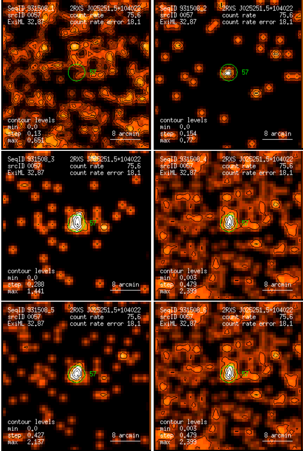
Figure 57: RASS 931508: detection 0057: band rate images, Gaussian filter: (1) PSPC channels 11 – 41, (2) 52 – 90, (3) 91 – 201, (4) 11 – 235, (5) 52 – 201, (6) 11 – 201. Broad band rates in counts/ks. Band rate contour levels in counts/ks/arcmin 2 .
