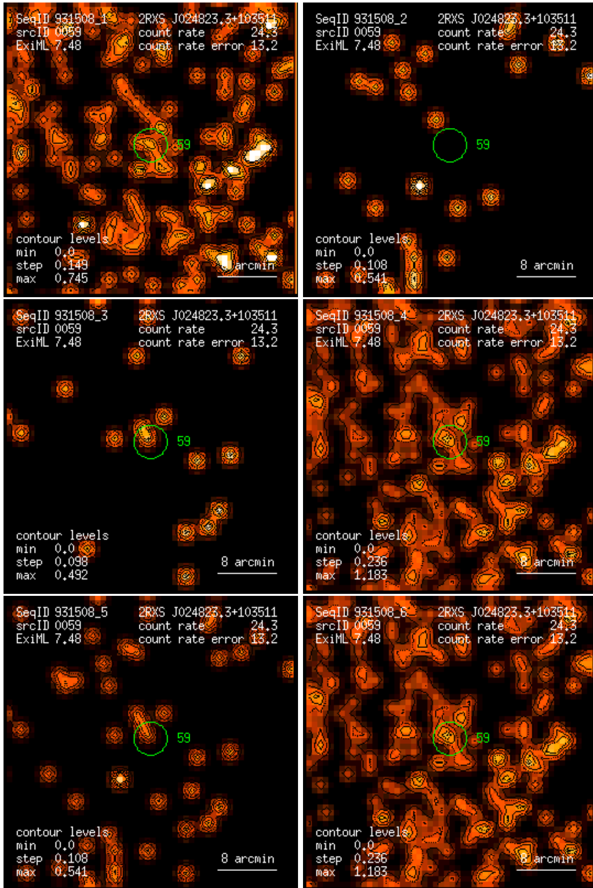
Figure 59: RASS 931508: detection 0059: band rate images, Gaussian filter: (1) PSPC channels 11 – 41, (2) 52 – 90, (3) 91 – 201, (4) 11 – 235, (5) 52 – 201, (6) 11 – 201. Broad band rates in counts/ks. Band rate contour levels in counts/ks/arcmin 2 .
