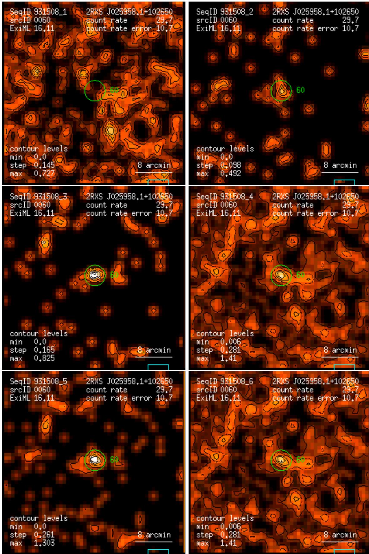
Figure 60: RASS 931508: detection 0060: band rate images, Gaussian filter: (1) PSPC channels 11 – 41, (2) 52 – 90, (3) 91 – 201, (4) 11 – 235, (5) 52 – 201, (6) 11 – 201. Broad band rates in counts/ks. Band rate contour levels in counts/ks/arcmin 2 .
