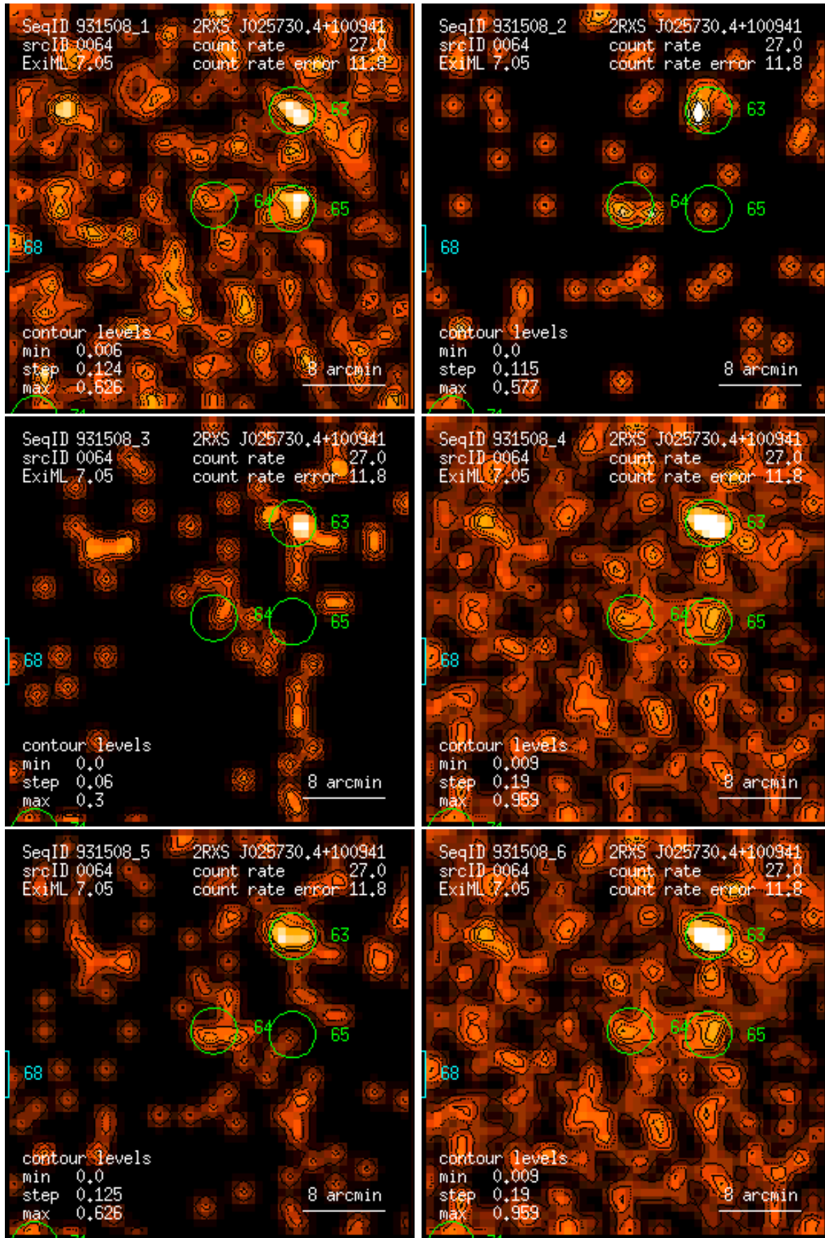
Figure 64: RASS 931508: detection 0064: band rate images, Gaussian filter: (1) PSPC channels 11 – 41, (2) 52 – 90, (3) 91 – 201, (4) 11 – 235, (5) 52 – 201, (6) 11 – 201. Broad band rates in counts/ks. Band rate contour levels in counts/ks/arcmin 2 .
