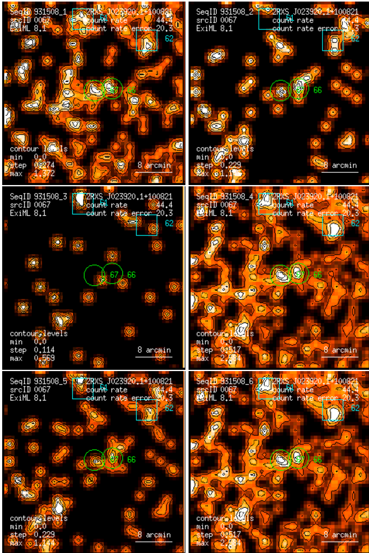
Figure 67: RASS 931508: detection 0067: band rate images, Gaussian filter: (1) PSPC channels 11 – 41, (2) 52 – 90, (3) 91 – 201, (4) 11 – 235, (5) 52 – 201, (6) 11 – 201. Broad band rates in counts/ks. Band rate contour levels in counts/ks/arcmin 2 .
