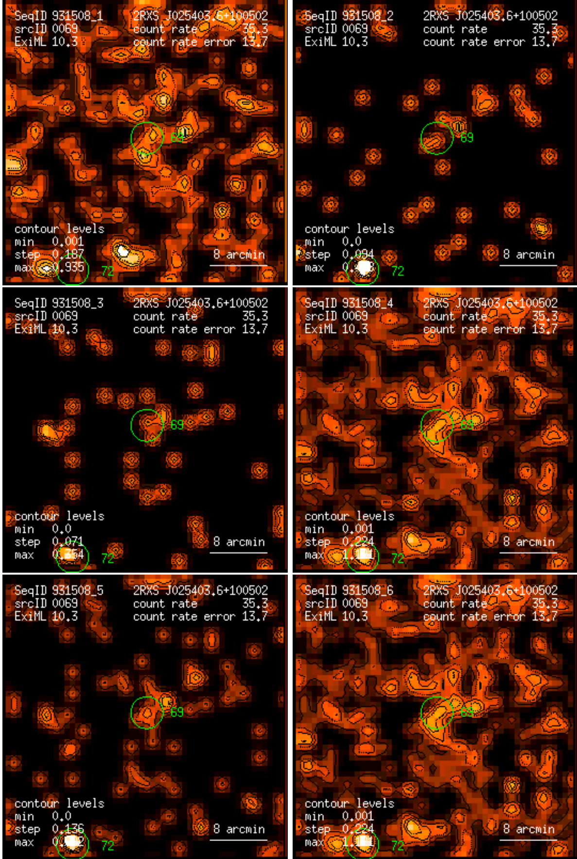
Figure 69: RASS 931508: detection 0069: band rate images, Gaussian filter: (1) PSPC channels 11 – 41, (2) 52 – 90, (3) 91 – 201, (4) 11 – 235, (5) 52 – 201, (6) 11 – 201. Broad band rates in counts/ks. Band rate contour levels in counts/ks/arcmin 2 .
