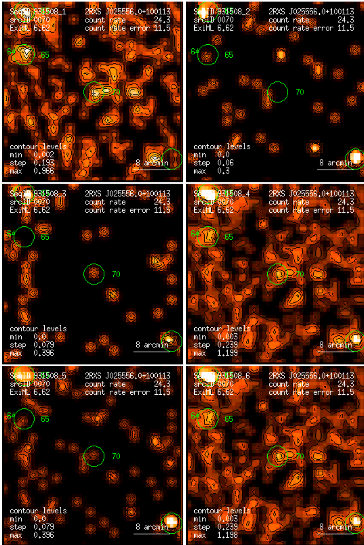
Figure 70: RASS 931508: detection 0070: band rate images, Gaussian filter: (1) PSPC channels 11 – 41, (2) 52 – 90, (3) 91 – 201, (4) 11 – 235, (5) 52 – 201, (6) 11 – 201. Broad band rates in counts/ks. Band rate contour levels in counts/ks/arcmin 2 .
