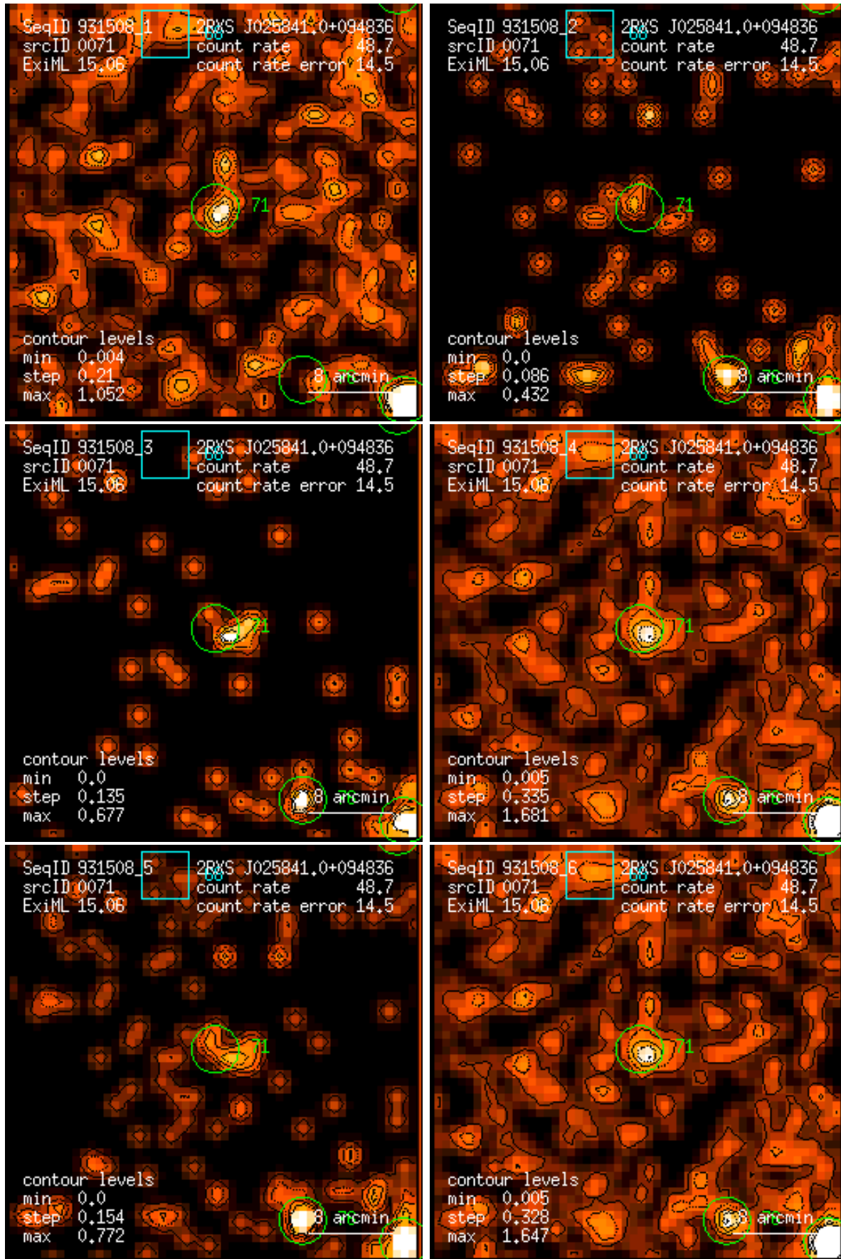
Figure 71: RASS 931508: detection 0071: band rate images, Gaussian filter: (1) PSPC channels 11 – 41, (2) 52 – 90, (3) 91 – 201, (4) 11 – 235, (5) 52 – 201, (6) 11 – 201. Broad band rates in counts/ks. Band rate contour levels in counts/ks/arcmin 2 .
