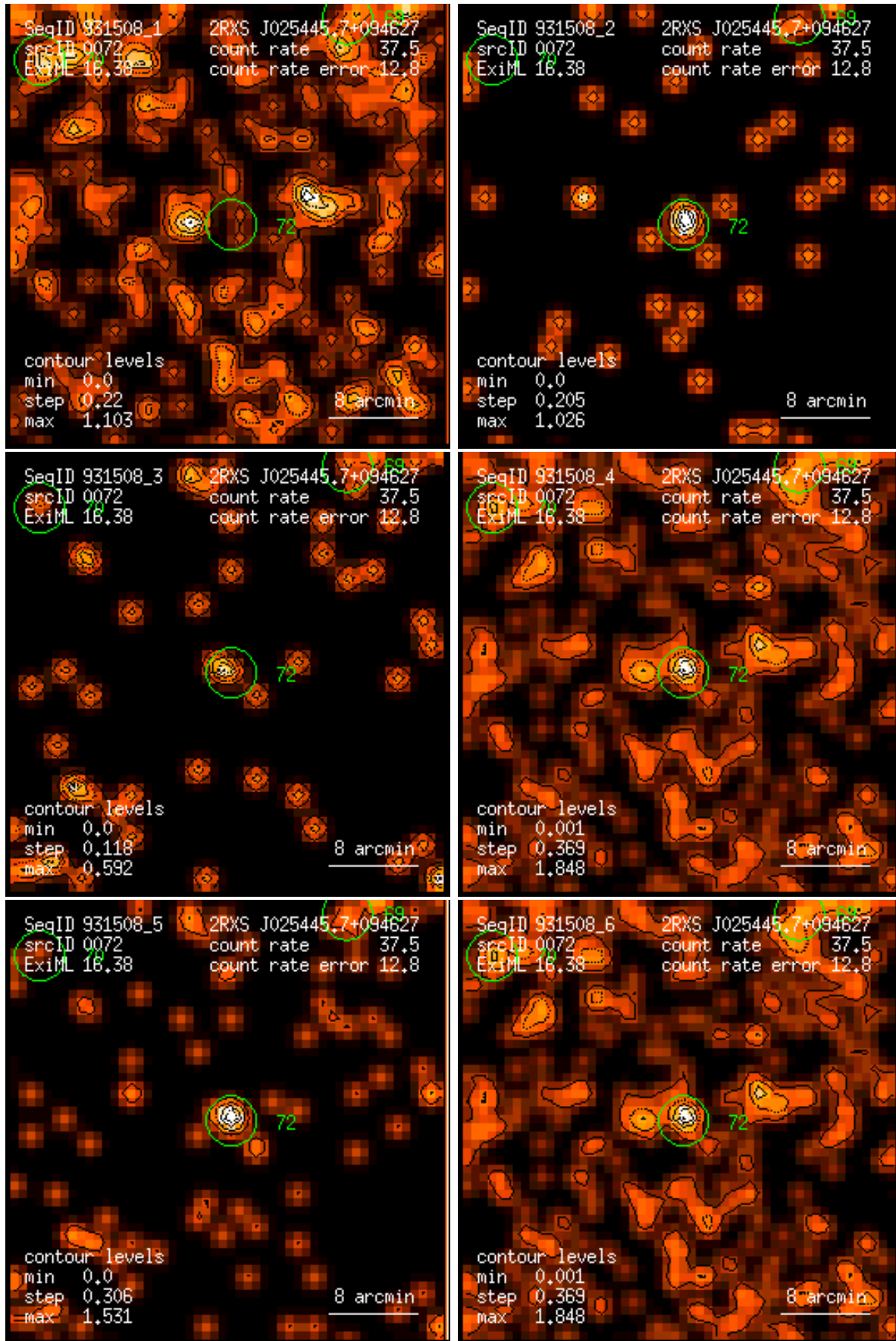
Figure 72: RASS 931508: detection 0072: band rate images, Gaussian filter: (1) PSPC channels 11 – 41, (2) 52 – 90, (3) 91 – 201, (4) 11 – 235, (5) 52 – 201, (6) 11 – 201. Broad band rates in counts/ks. Band rate contour levels in counts/ks/arcmin 2 .
