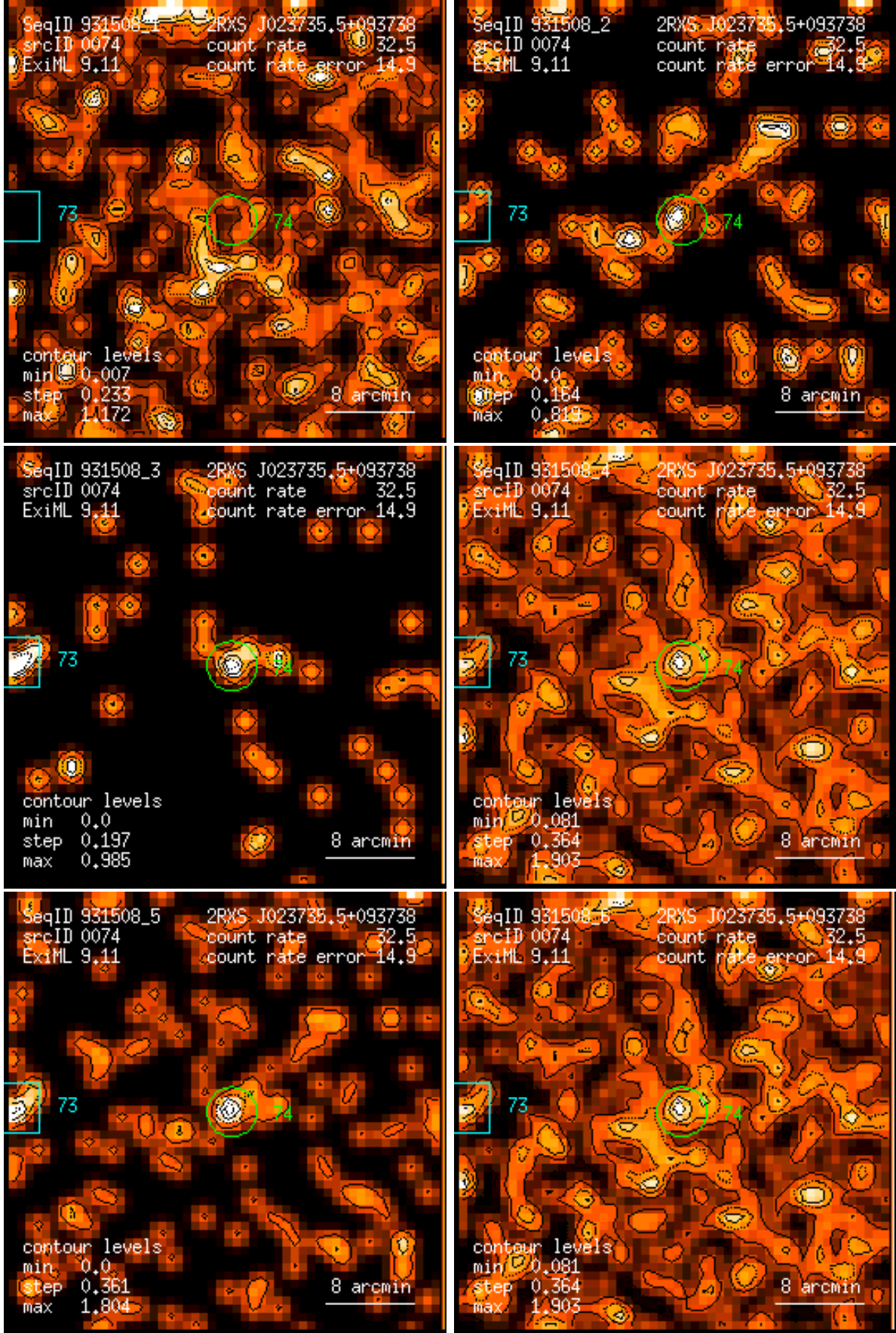
Figure 74: RASS 931508: detection 0074: band rate images, Gaussian filter: (1) PSPC channels 11 – 41, (2) 52 – 90, (3) 91 – 201, (4) 11 – 235, (5) 52 – 201, (6) 11 – 201. Broad band rates in counts/ks. Band rate contour levels in counts/ks/arcmin 2 .
