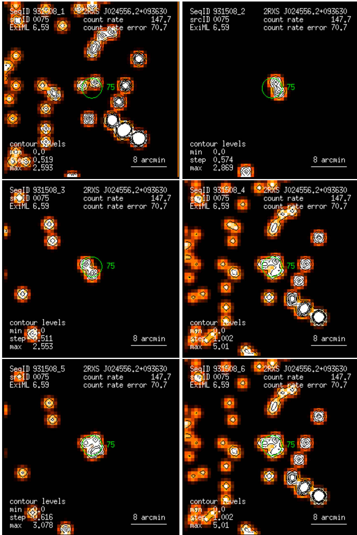
Figure 75: RASS 931508: detection 0075: band rate images, Gaussian filter: (1) PSPC channels 11 – 41, (2) 52 – 90, (3) 91 – 201, (4) 11 – 235, (5) 52 – 201, (6) 11 – 201. Broad band rates in counts/ks. Band rate contour levels in counts/ks/arcmin 2 .
