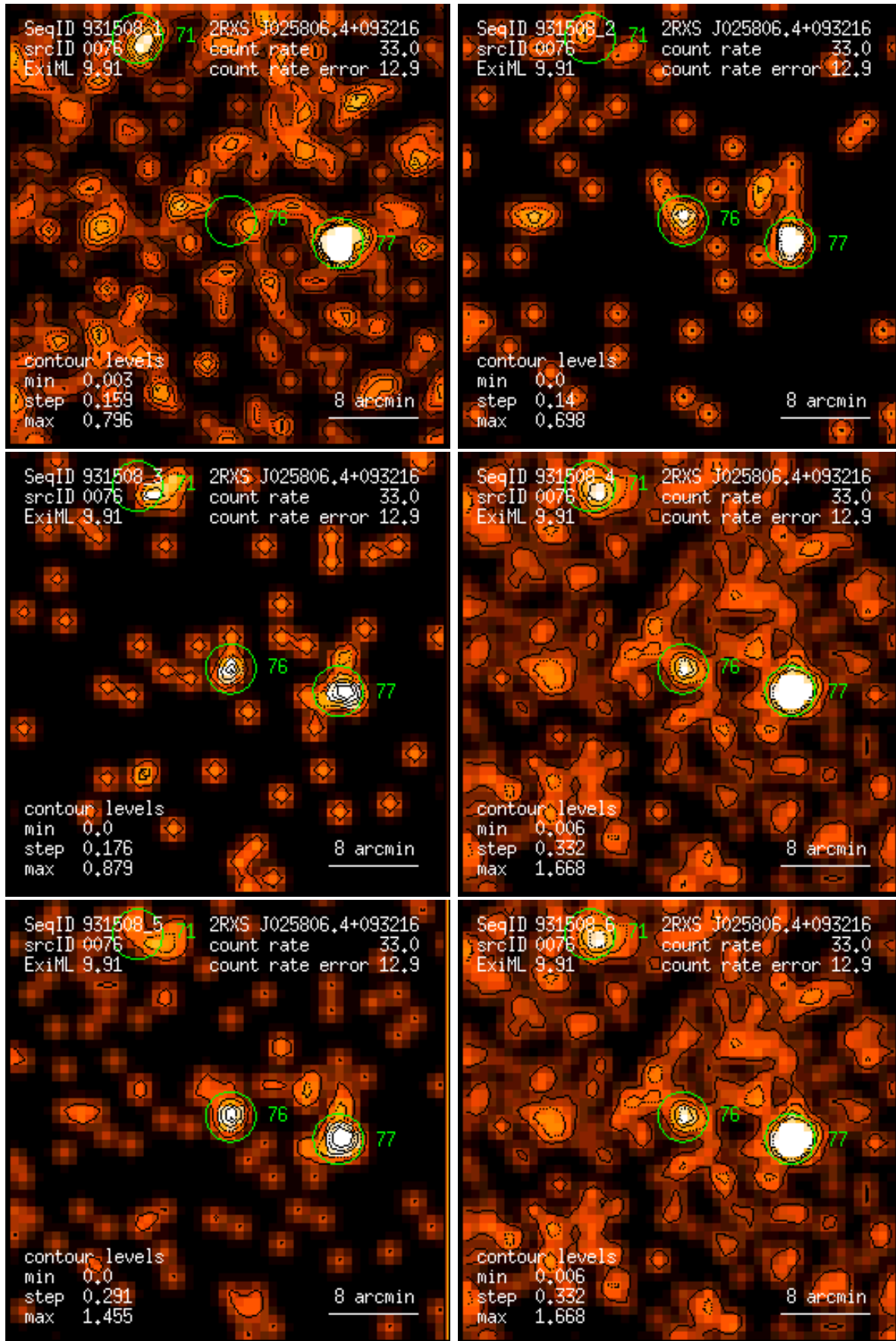
Figure 76: RASS 931508: detection 0076: band rate images, Gaussian filter: (1) PSPC channels 11 – 41, (2) 52 – 90, (3) 91 – 201, (4) 11 – 235, (5) 52 – 201, (6) 11 – 201. Broad band rates in counts/ks. Band rate contour levels in counts/ks/arcmin 2 .
