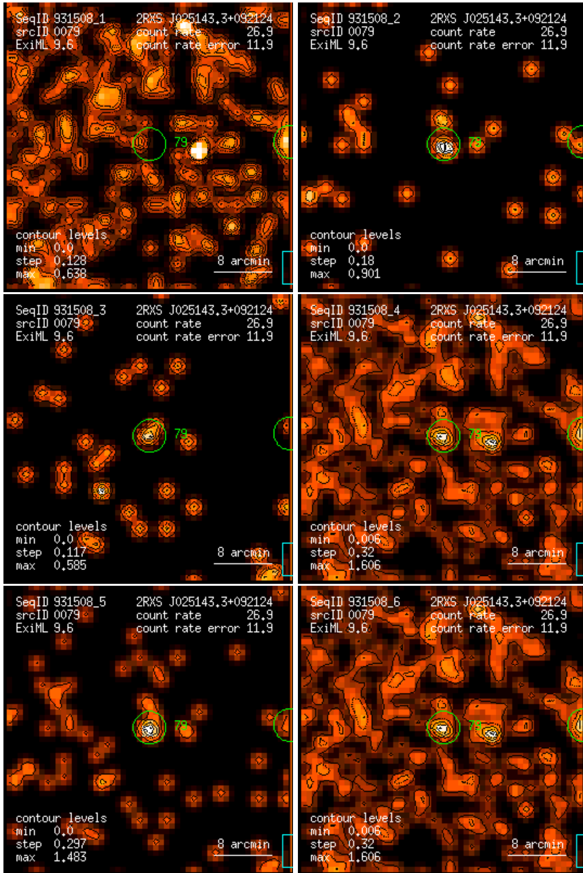
Figure 79: RASS 931508: detection 0079: band rate images, Gaussian filter: (1) PSPC channels 11 – 41, (2) 52 – 90, (3) 91 – 201, (4) 11 – 235, (5) 52 – 201, (6) 11 – 201. Broad band rates in counts/ks. Band rate contour levels in counts/ks/arcmin 2 .
