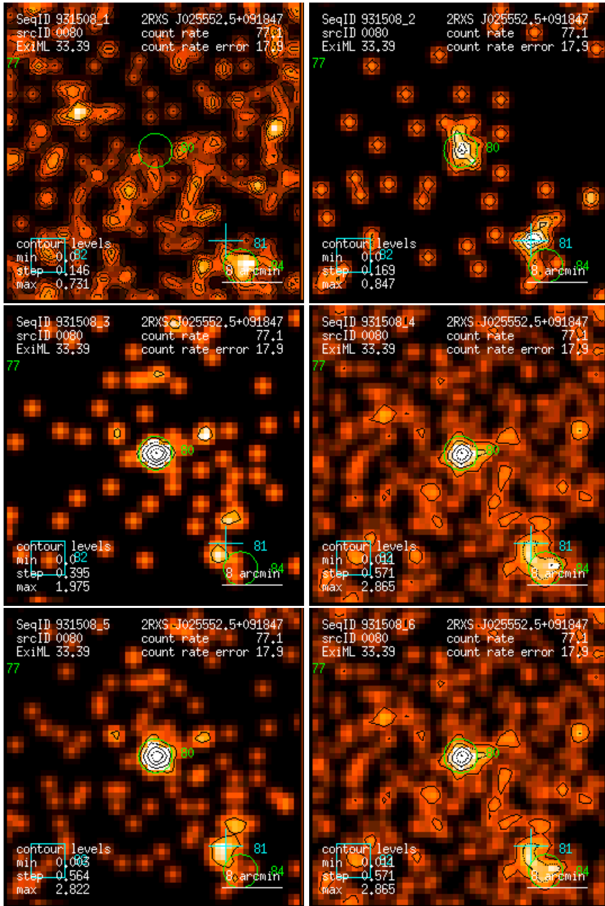
Figure 80: RASS 931508: detection 0080: band rate images, Gaussian filter: (1) PSPC channels 11 – 41, (2) 52 – 90, (3) 91 – 201, (4) 11 – 235, (5) 52 – 201, (6) 11 – 201. Broad band rates in counts/ks. Band rate contour levels in counts/ks/arcmin 2 .
