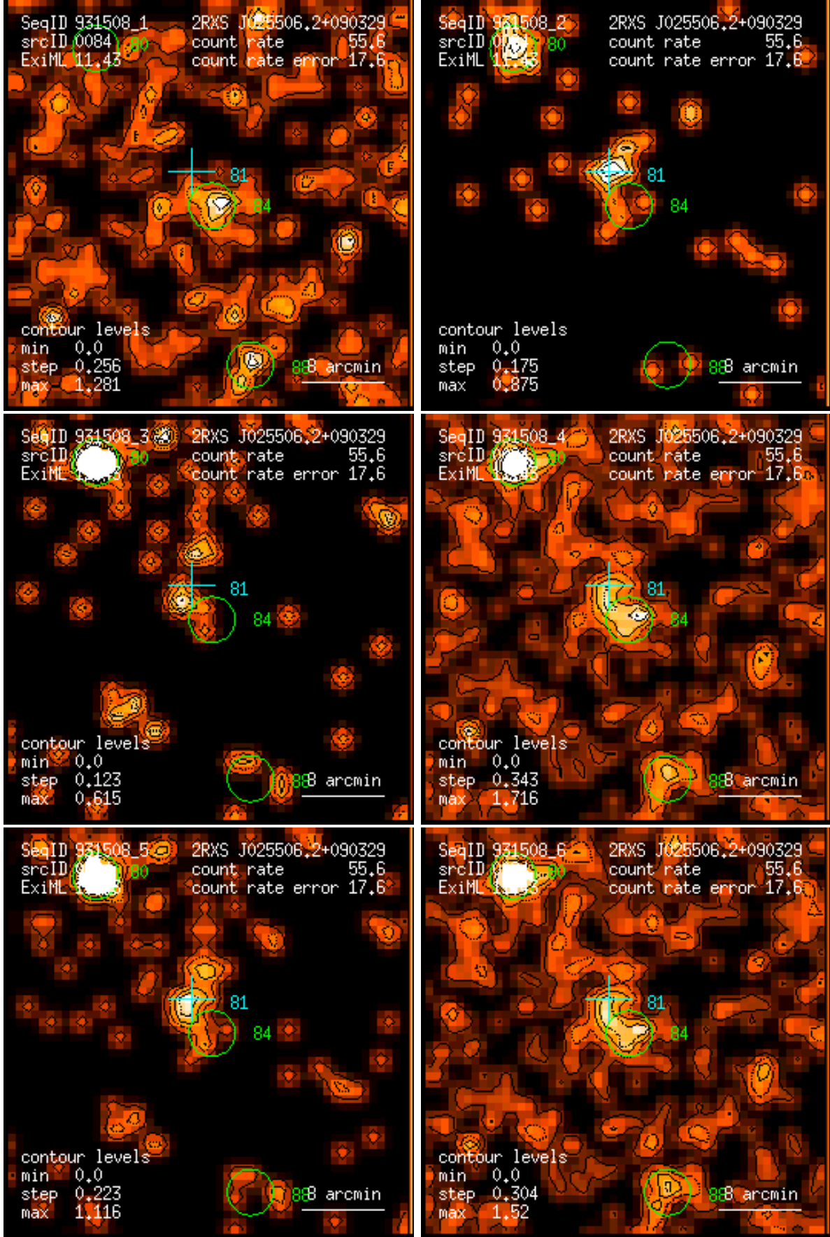
Figure 84: RASS 931508: detection 0084: band rate images, Gaussian filter: (1) PSPC channels 11 – 41, (2) 52 – 90, (3) 91 – 201, (4) 11 – 235, (5) 52 – 201, (6) 11 – 201. Broad band rates in counts/ks. Band rate contour levels in counts/ks/arcmin 2 .
