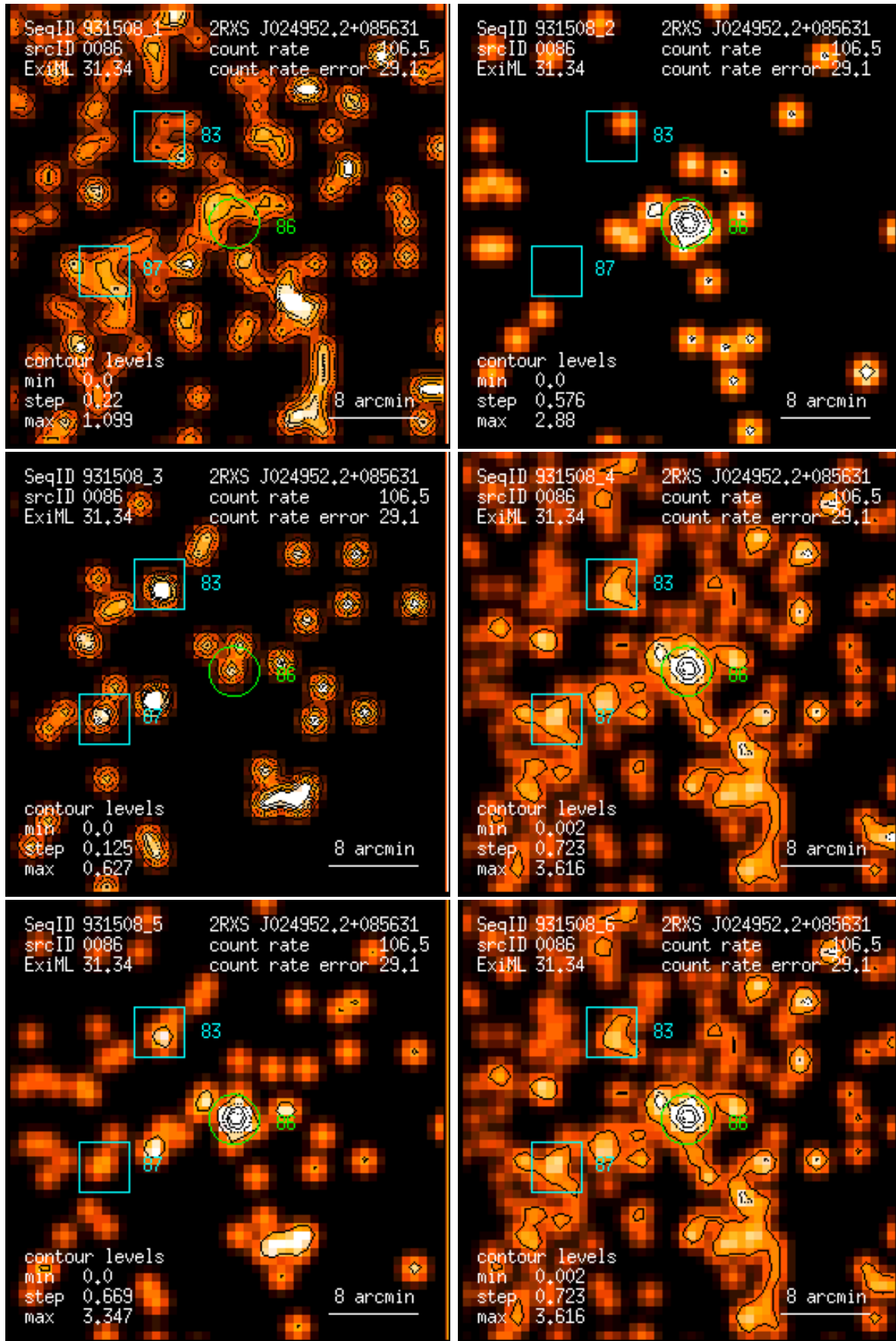
Figure 86: RASS 931508: detection 0086: band rate images, Gaussian filter: (1) PSPC channels 11 – 41, (2) 52 – 90, (3) 91 – 201, (4) 11 – 235, (5) 52 – 201, (6) 11 – 201. Broad band rates in counts/ks. Band rate contour levels in counts/ks/arcmin 2 .
