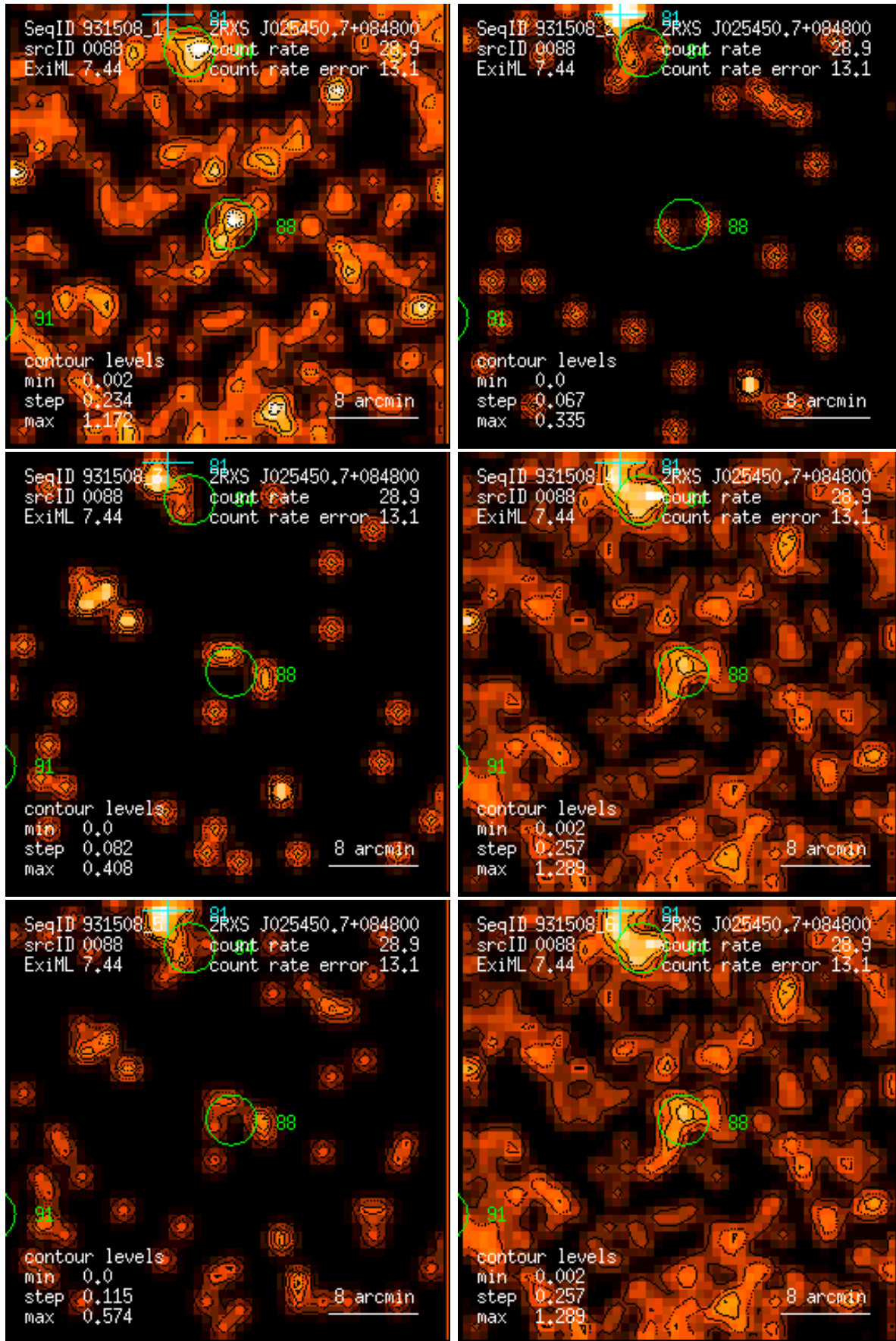
Figure 88: RASS 931508: detection 0088: band rate images, Gaussian filter: (1) PSPC channels 11 – 41, (2) 52 – 90, (3) 91 – 201, (4) 11 – 235, (5) 52 – 201, (6) 11 – 201. Broad band rates in counts/ks. Band rate contour levels in counts/ks/arcmin 2 .
