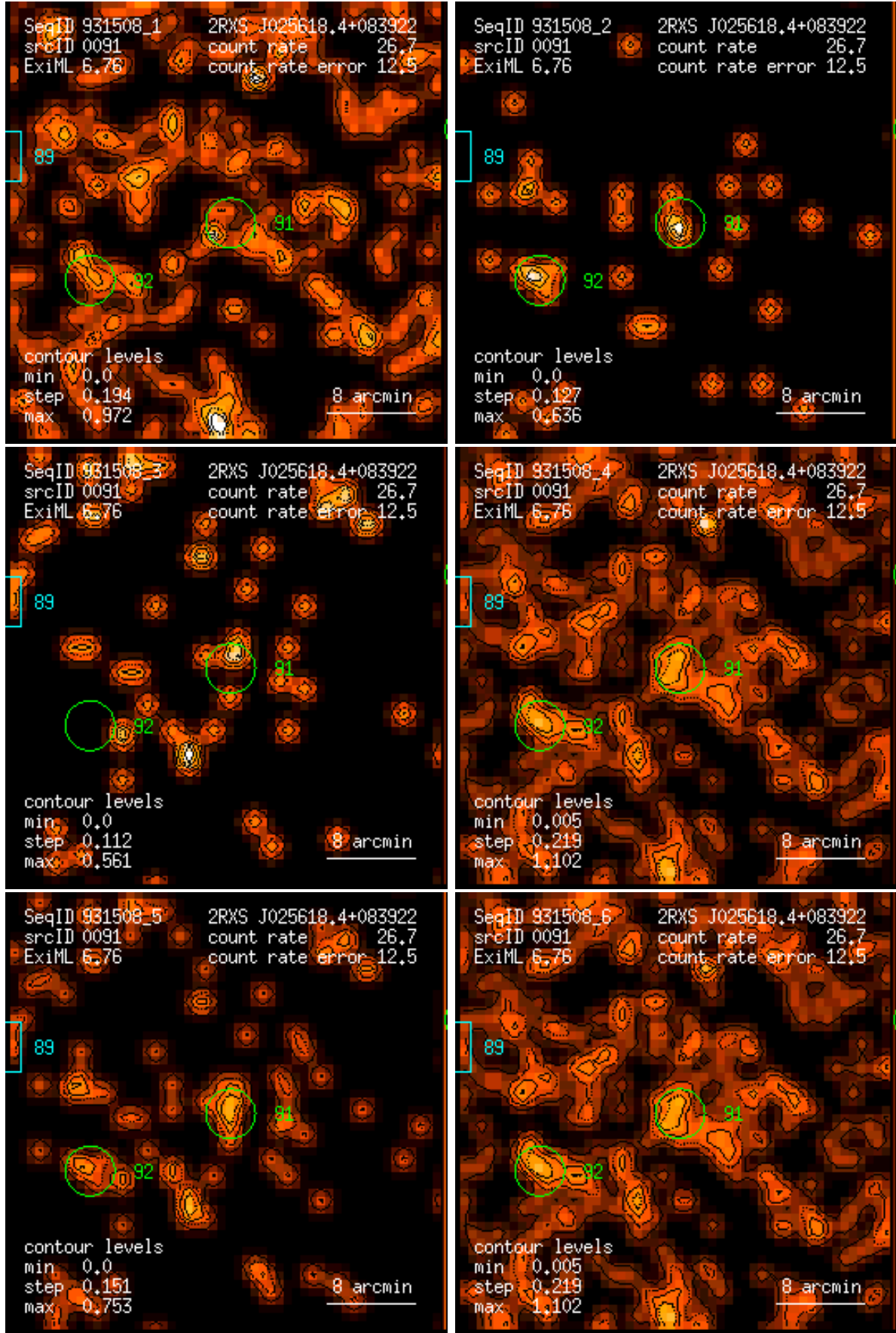
Figure 91: RASS 931508: detection 0091: band rate images, Gaussian filter: (1) PSPC channels 11 – 41, (2) 52 – 90, (3) 91 – 201, (4) 11 – 235, (5) 52 – 201, (6) 11 – 201. Broad band rates in counts/ks. Band rate contour levels in counts/ks/arcmin 2 .
