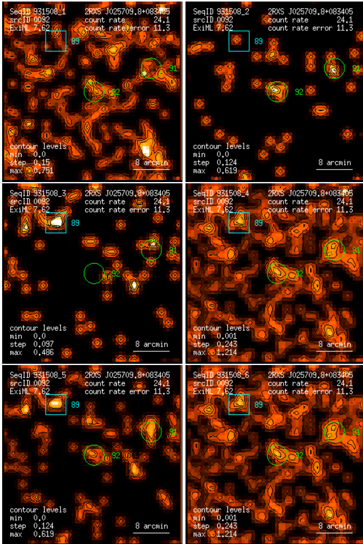
Figure 92: RASS 931508: detection 0092: band rate images, Gaussian filter: (1) PSPC channels 11 – 41, (2) 52 – 90, (3) 91 – 201, (4) 11 – 235, (5) 52 – 201, (6) 11 – 201. Broad band rates in counts/ks. Band rate contour levels in counts/ks/arcmin 2 .
