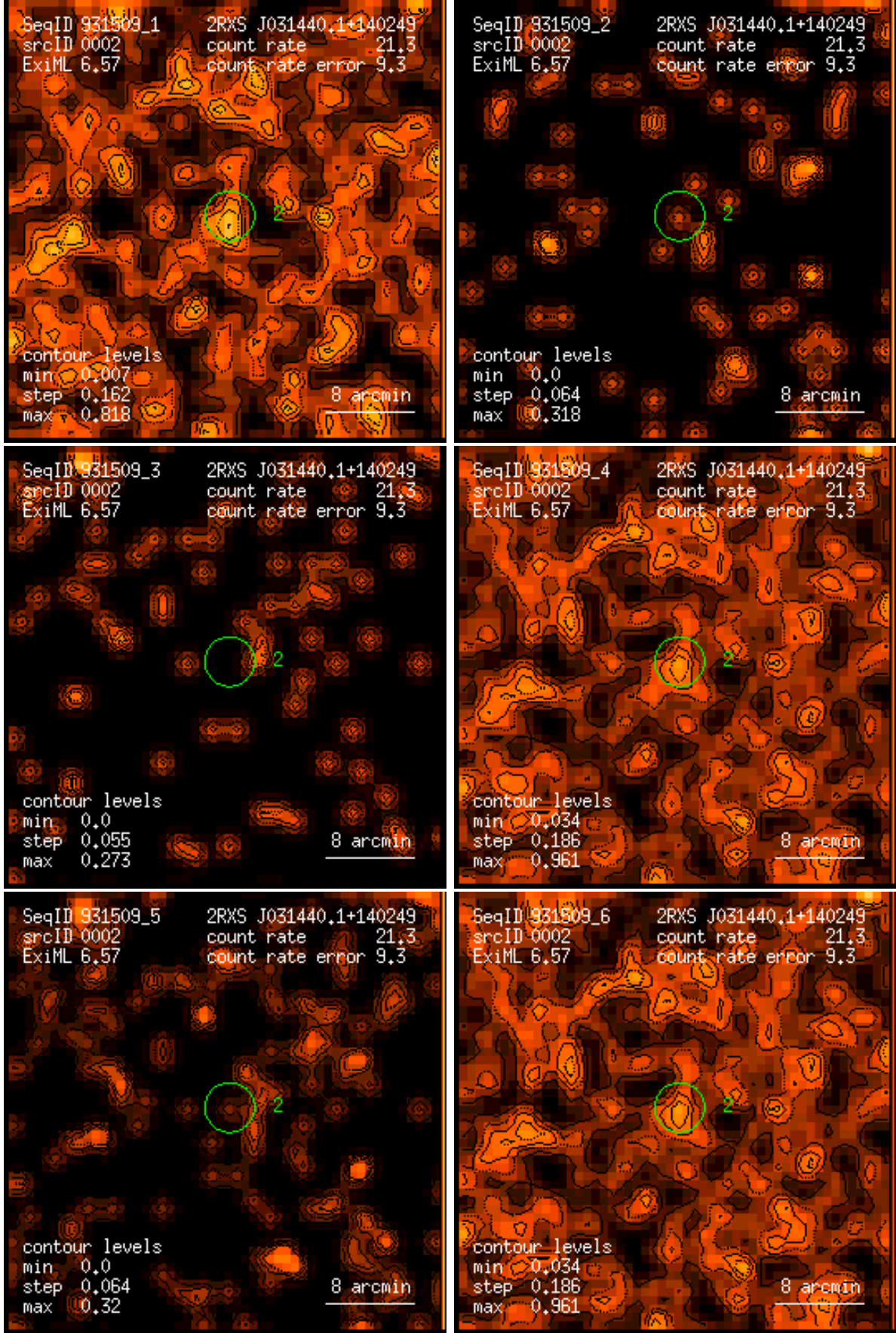
Figure 2: RASS 931509: detection 0002: band rate images, Gaussian filter: (1) PSPC channels 11 – 41, (2) 52 – 90, (3) 91 – 201, (4) 11 – 235, (5) 52 – 201, (6) 11 – 201. Broad band rates in counts/ks. Band rate contour levels in counts/ks/arcmin 2 .
