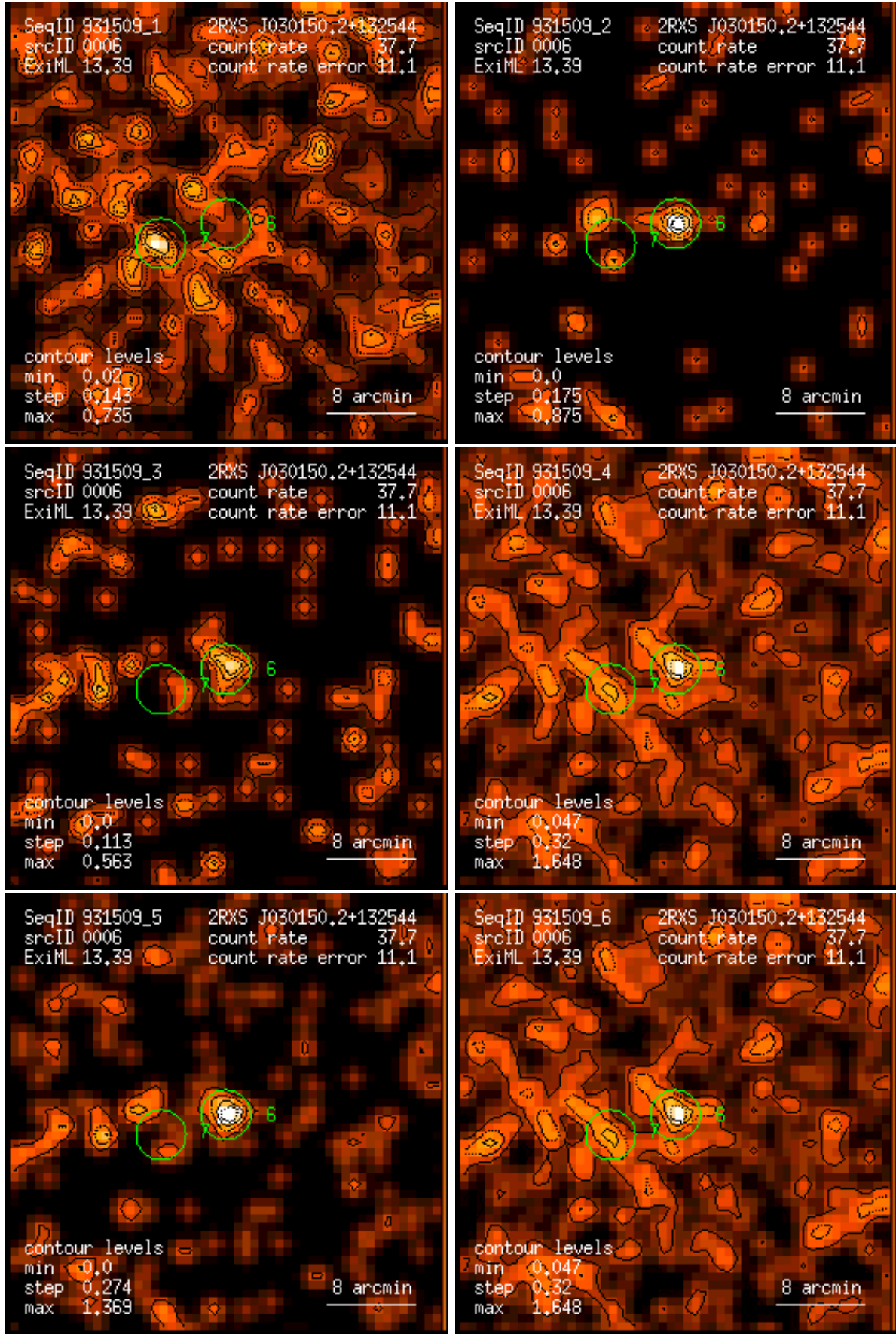
Figure 6: RASS 931509: detection 0006: band rate images, Gaussian filter: (1) PSPC channels 11 – 41, (2) 52 – 90, (3) 91 – 201, (4) 11 – 235, (5) 52 – 201, (6) 11 – 201. Broad band rates in counts/ks. Band rate contour levels in counts/ks/arcmin 2 .
