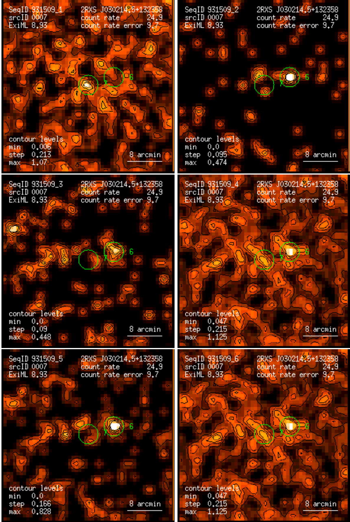
Figure 7: RASS 931509: detection 0007: band rate images, Gaussian filter: (1) PSPC channels 11 – 41, (2) 52 – 90, (3) 91 – 201, (4) 11 – 235, (5) 52 – 201, (6) 11 – 201. Broad band rates in counts/ks. Band rate contour levels in counts/ks/arcmin 2 .
