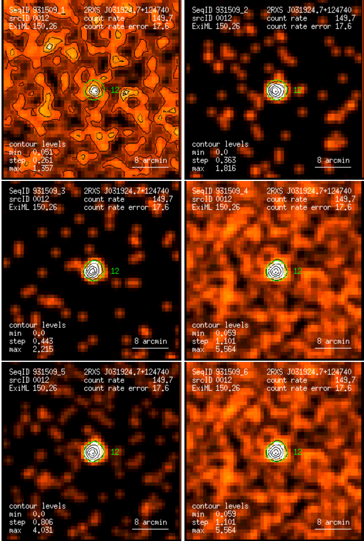
Figure 12: RASS 931509: detection 0012: band rate images, Gaussian filter: (1) PSPC channels 11 – 41, (2) 52 – 90, (3) 91 – 201, (4) 11 – 235, (5) 52 – 201, (6) 11 – 201. Broad band rates in counts/ks. Band rate contour levels in counts/ks/arcmin 2 .
