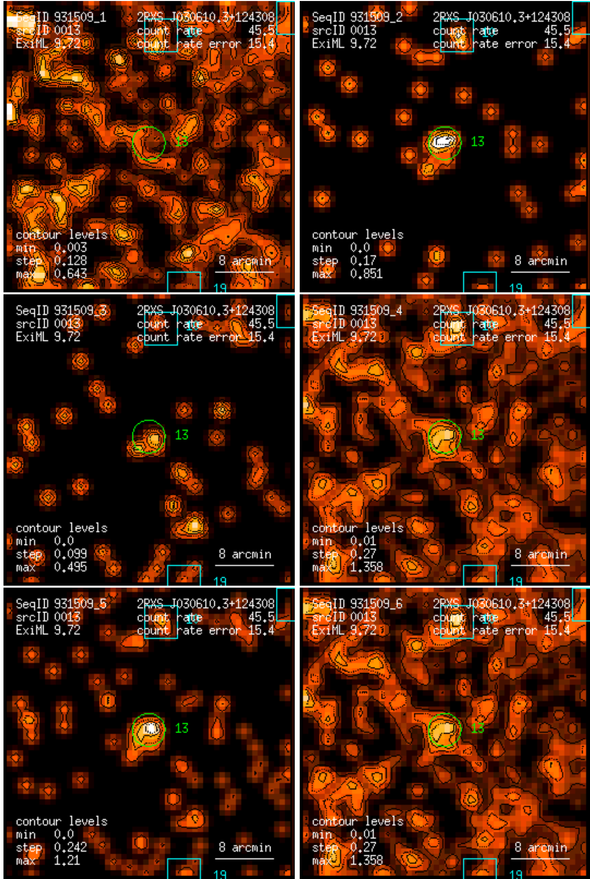
Figure 13: RASS 931509: detection 0013: band rate images, Gaussian filter: (1) PSPC channels 11 – 41, (2) 52 – 90, (3) 91 – 201, (4) 11 – 235, (5) 52 – 201, (6) 11 – 201. Broad band rates in counts/ks. Band rate contour levels in counts/ks/arcmin 2 .
