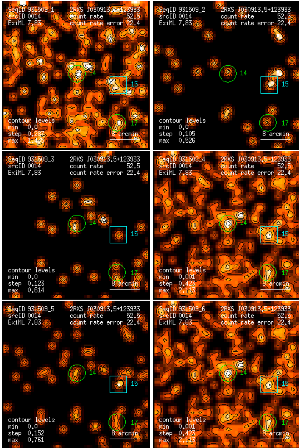
Figure 14: RASS 931509: detection 0014: band rate images, Gaussian filter: (1) PSPC channels 11 – 41, (2) 52 – 90, (3) 91 – 201, (4) 11 – 235, (5) 52 – 201, (6) 11 – 201. Broad band rates in counts/ks. Band rate contour levels in counts/ks/arcmin 2 .
